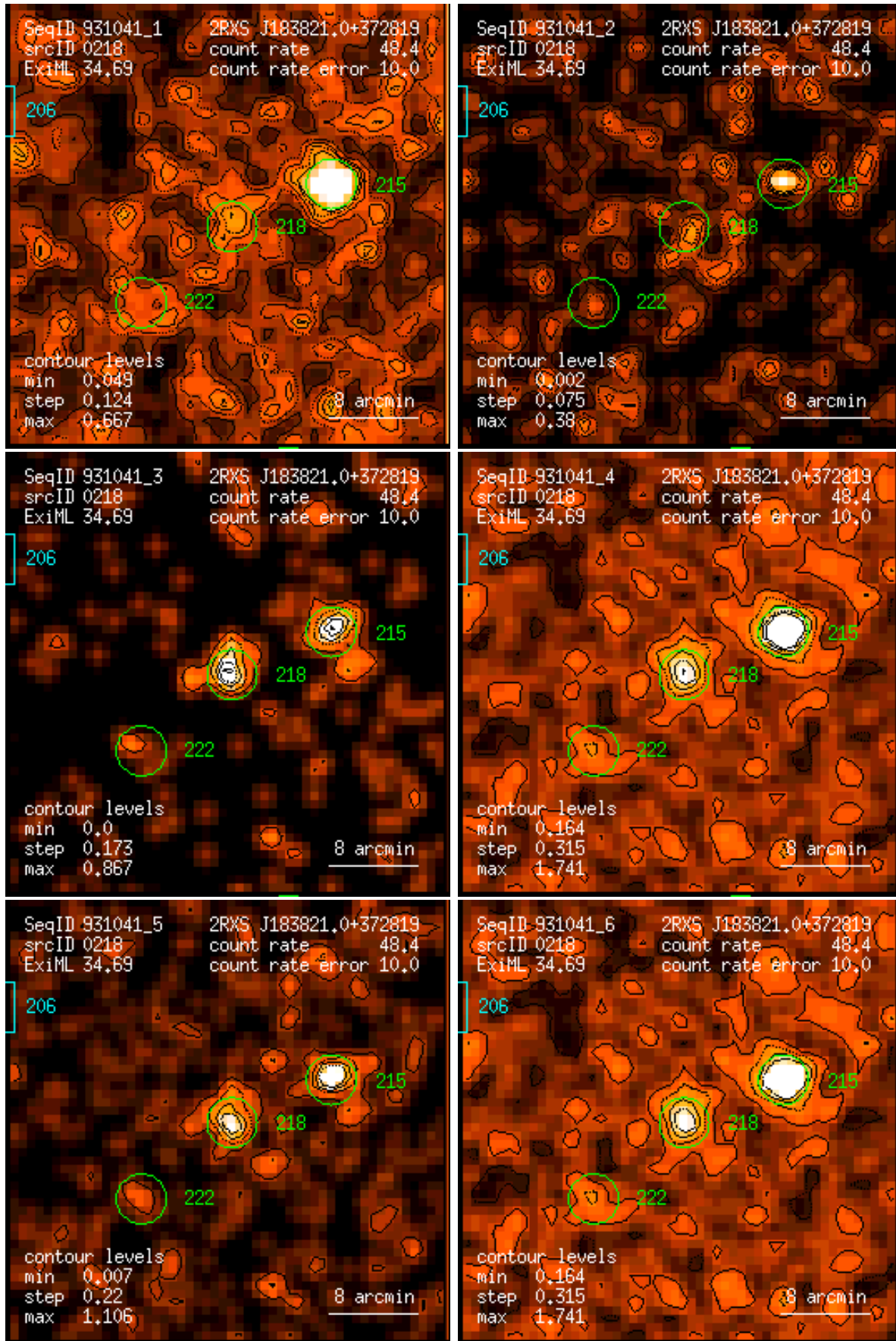
Figure 218: RASS 931041: detection 0218: band rate images, Gaussian filter: (1) PSPC channels 11 – 41, (2) 52 – 90, (3) 91 – 201, (4) 11 – 235, (5) 52 – 201, (6) 11 – 201. Broad band rates in counts/ks. Band rate contour levels in counts/ks/arcmin 2 .
