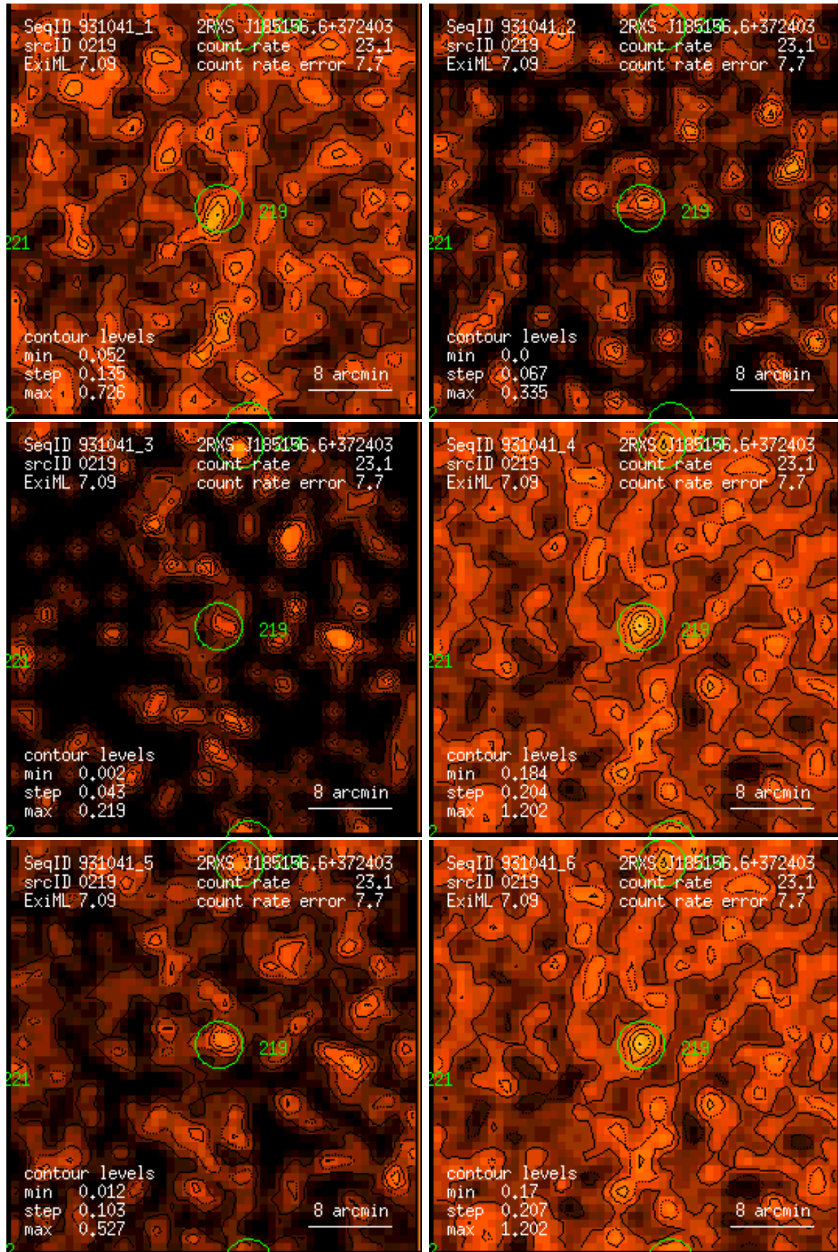
Figure 219: RASS 931041: detection 0219: band rate images, Gaussian filter: (1) PSPC channels 11 – 41, (2) 52 – 90, (3) 91 – 201, (4) 11 – 235, (5) 52 – 201, (6) 11 – 201. Broad band rates in counts/ks. Band rate contour levels in counts/ks/arcmin 2 .
