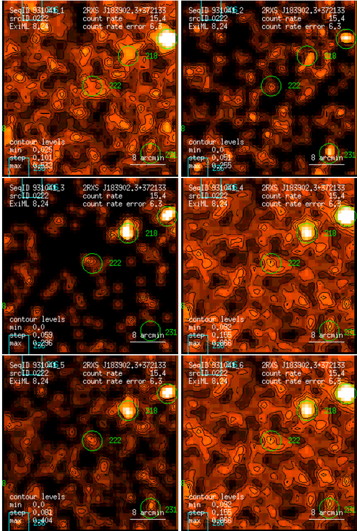
Figure 222: RASS 931041: detection 0222: band rate images, Gaussian filter: (1) PSPC channels 11 – 41, (2) 52 – 90, (3) 91 – 201, (4) 11 – 235, (5) 52 – 201, (6) 11 – 201. Broad band rates in counts/ks. Band rate contour levels in counts/ks/arcmin 2 .
