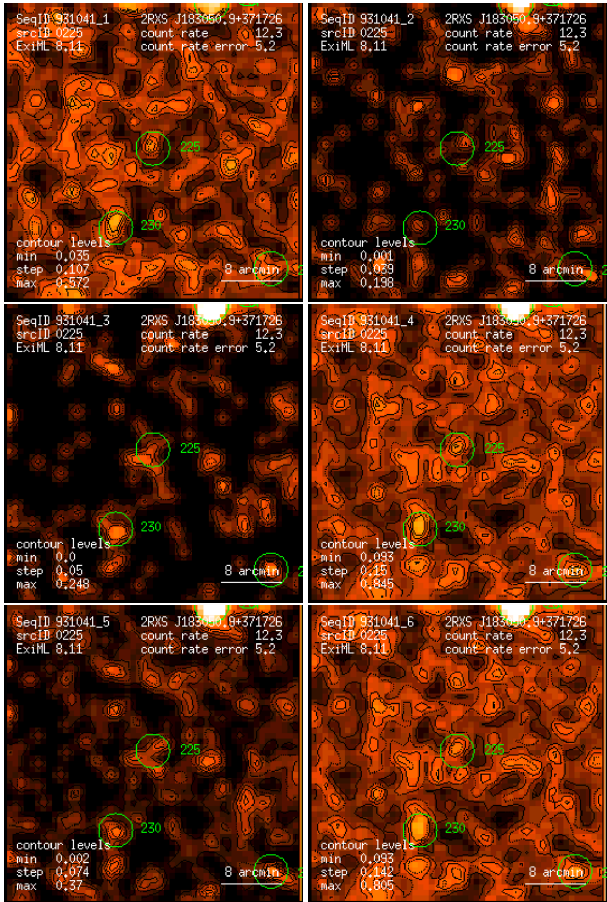
Figure 225: RASS 931041: detection 0225: band rate images, Gaussian filter: (1) PSPC channels 11 – 41, (2) 52 – 90, (3) 91 – 201, (4) 11 – 235, (5) 52 – 201, (6) 11 – 201. Broad band rates in counts/ks. Band rate contour levels in counts/ks/arcmin 2 .
