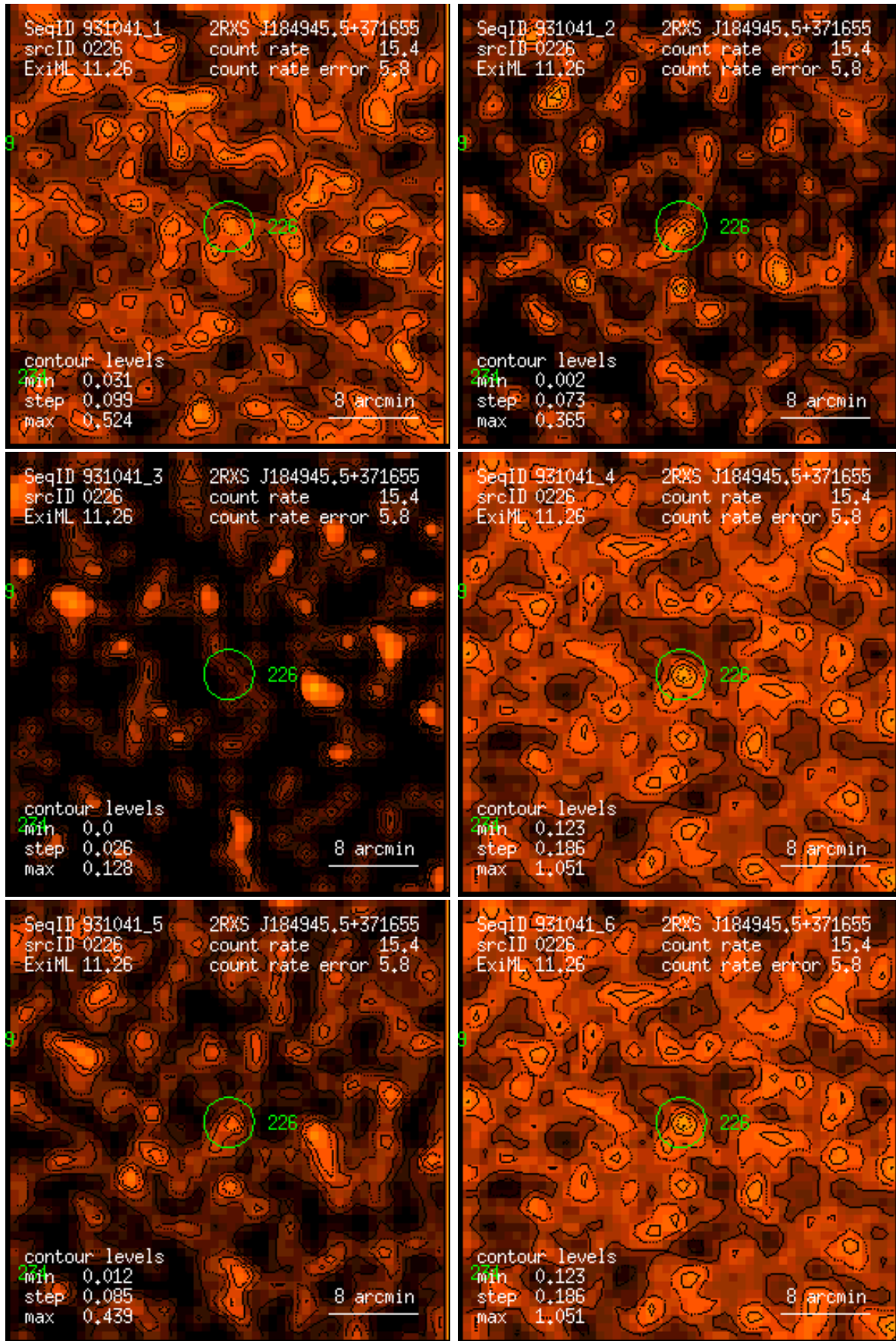
Figure 226: RASS 931041: detection 0226: band rate images, Gaussian filter: (1) PSPC channels 11 – 41, (2) 52 – 90, (3) 91 – 201, (4) 11 – 235, (5) 52 – 201, (6) 11 – 201. Broad band rates in counts/ks. Band rate contour levels in counts/ks/arcmin 2 .
