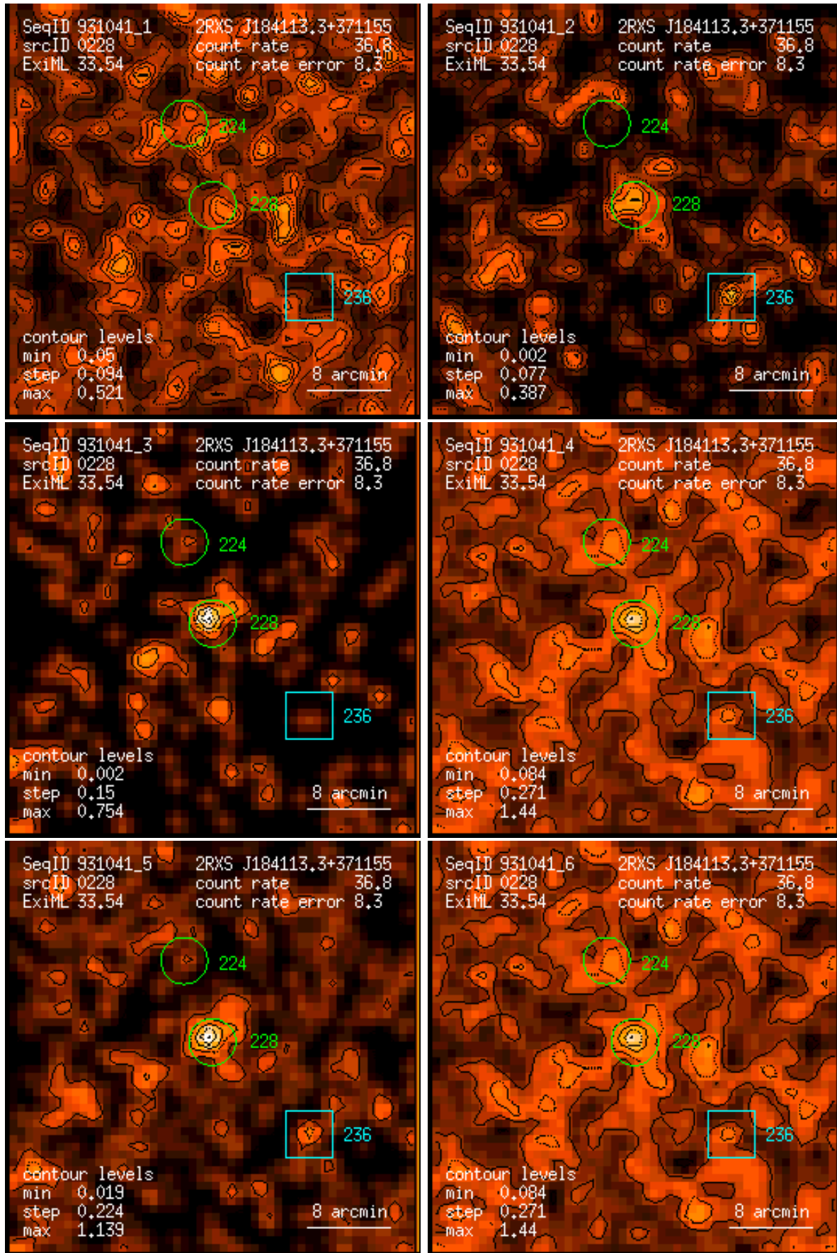
Figure 228: RASS 931041: detection 0228: band rate images, Gaussian filter: (1) PSPC channels 11 – 41, (2) 52 – 90, (3) 91 – 201, (4) 11 – 235, (5) 52 – 201, (6) 11 – 201. Broad band rates in counts/ks. Band rate contour levels in counts/ks/arcmin 2 .
