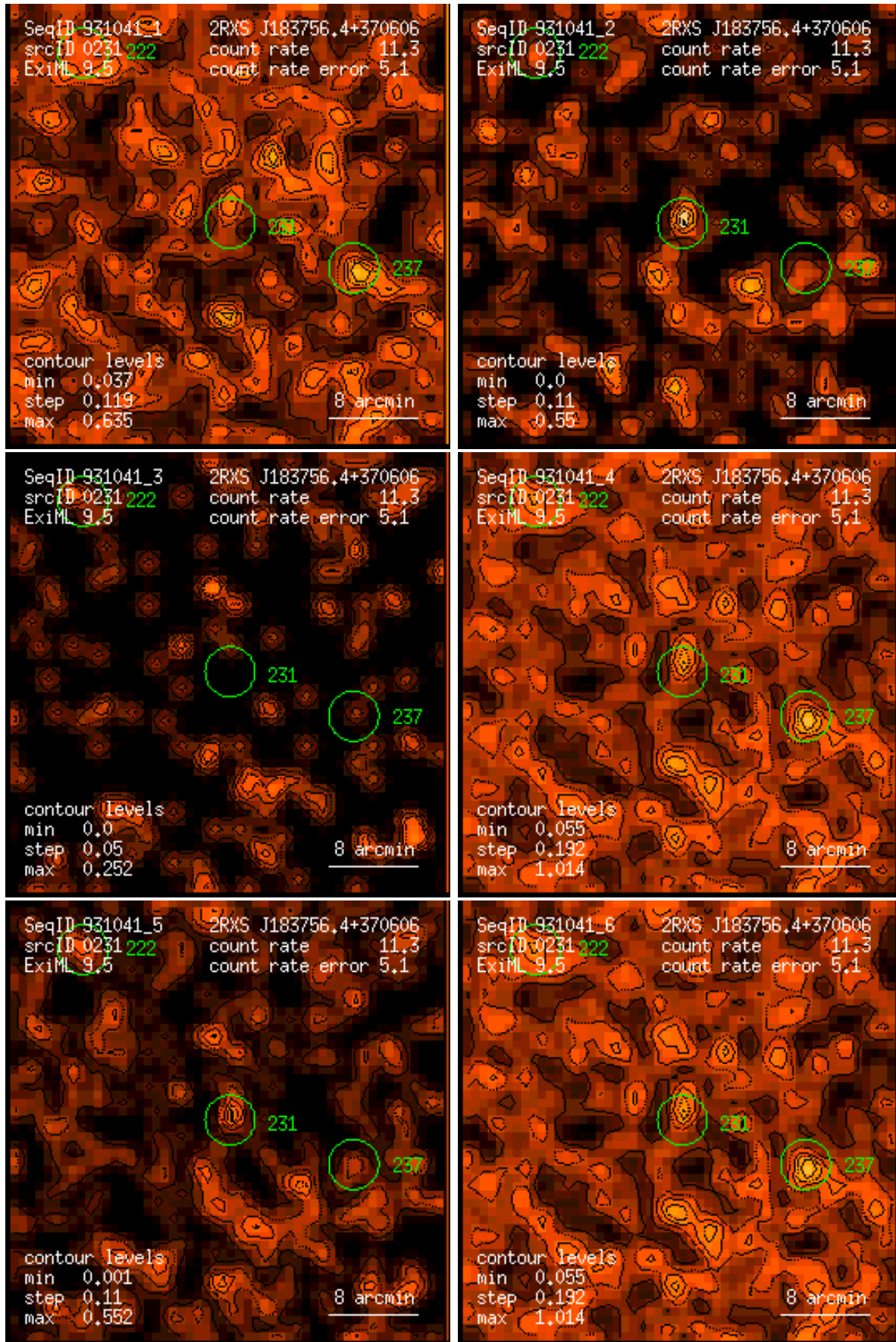
Figure 231: RASS 931041: detection 0231: band rate images, Gaussian filter: (1) PSPC channels 11 – 41, (2) 52 – 90, (3) 91 – 201, (4) 11 – 235, (5) 52 – 201, (6) 11 – 201. Broad band rates in counts/ks. Band rate contour levels in counts/ks/arcmin 2 .
