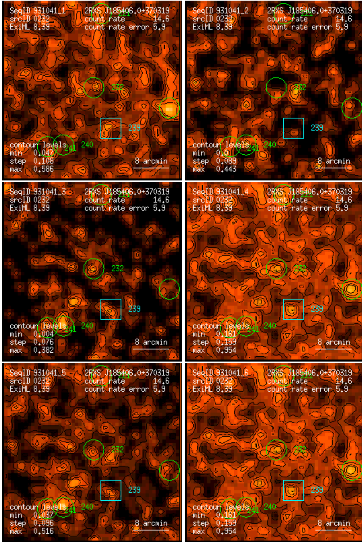
Figure 232: RASS 931041: detection 0232: band rate images, Gaussian filter: (1) PSPC channels 11 – 41, (2) 52 – 90, (3) 91 – 201, (4) 11 – 235, (5) 52 – 201, (6) 11 – 201. Broad band rates in counts/ks. Band rate contour levels in counts/ks/arcmin 2 .
