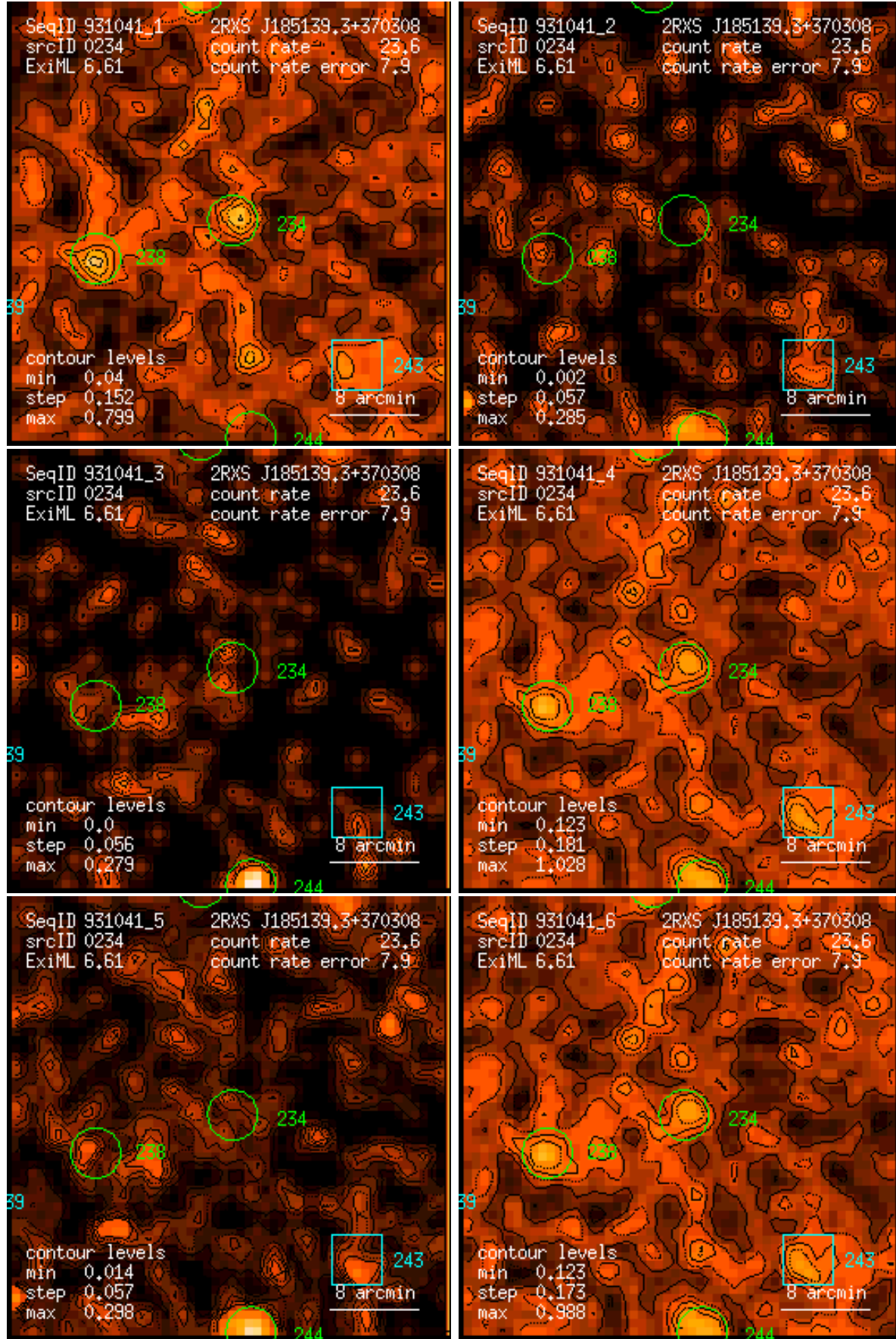
Figure 234: RASS 931041: detection 0234: band rate images, Gaussian filter: (1) PSPC channels 11 – 41, (2) 52 – 90, (3) 91 – 201, (4) 11 – 235, (5) 52 – 201, (6) 11 – 201. Broad band rates in counts/ks. Band rate contour levels in counts/ks/arcmin 2 .
