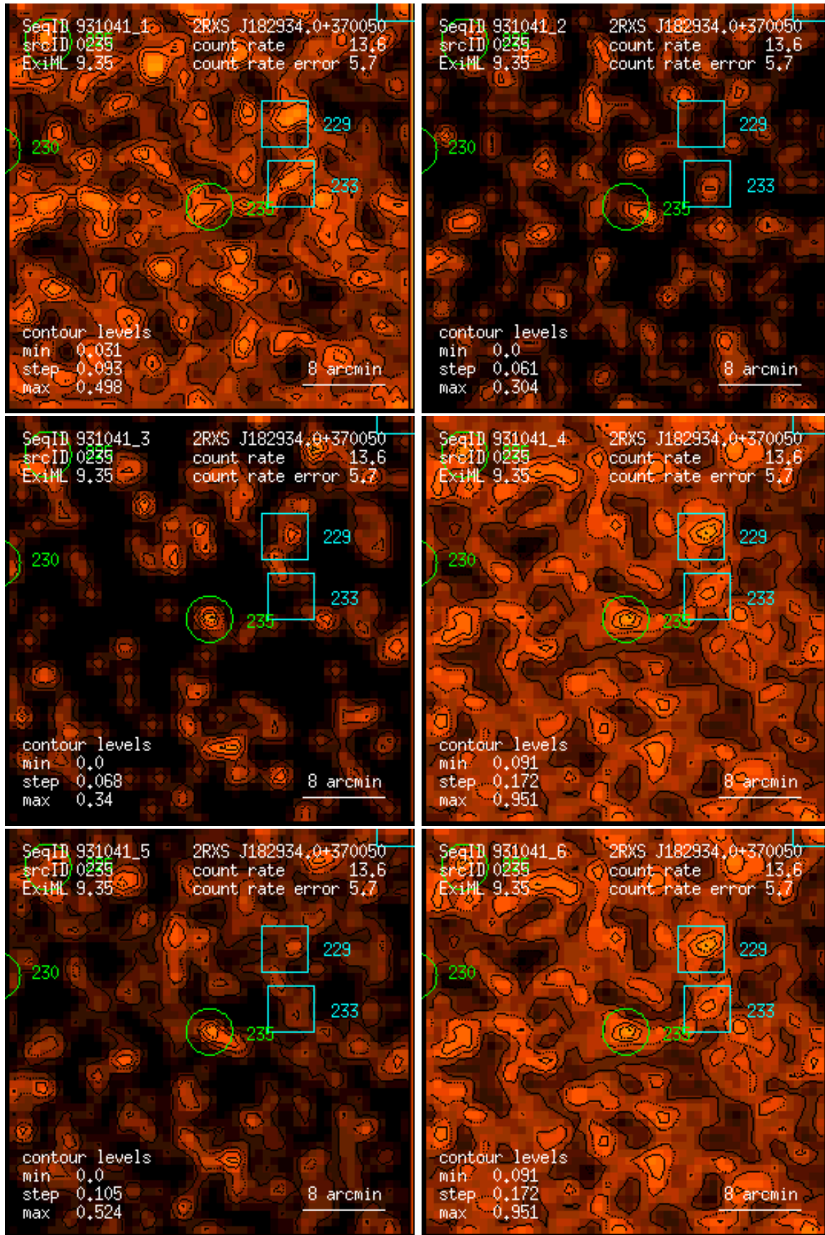
Figure 235: RASS 931041: detection 0235: band rate images, Gaussian filter: (1) PSPC channels 11 – 41, (2) 52 – 90, (3) 91 – 201, (4) 11 – 235, (5) 52 – 201, (6) 11 – 201. Broad band rates in counts/ks. Band rate contour levels in counts/ks/arcmin 2 .
