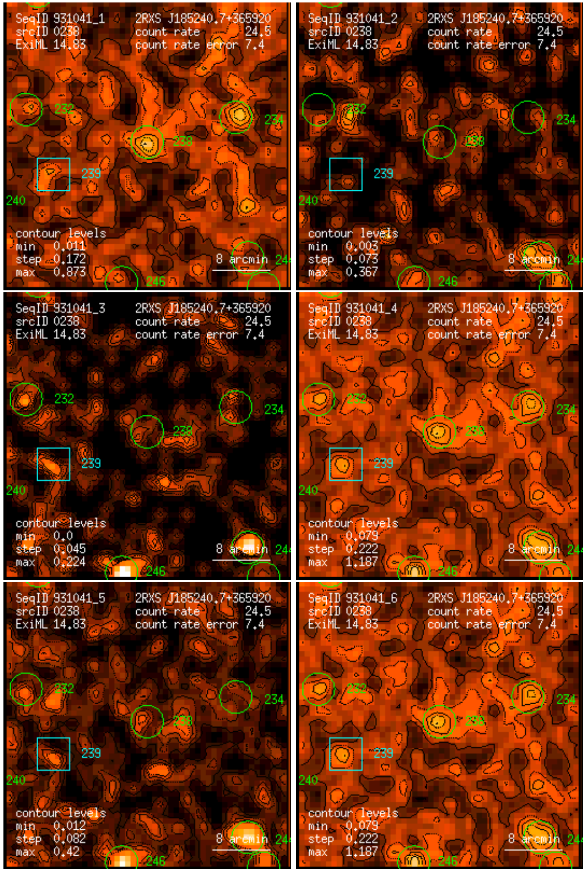
Figure 238: RASS 931041: detection 0238: band rate images, Gaussian filter: (1) PSPC channels 11 – 41, (2) 52 – 90, (3) 91 – 201, (4) 11 – 235, (5) 52 – 201, (6) 11 – 201. Broad band rates in counts/ks. Band rate contour levels in counts/ks/arcmin 2 .
