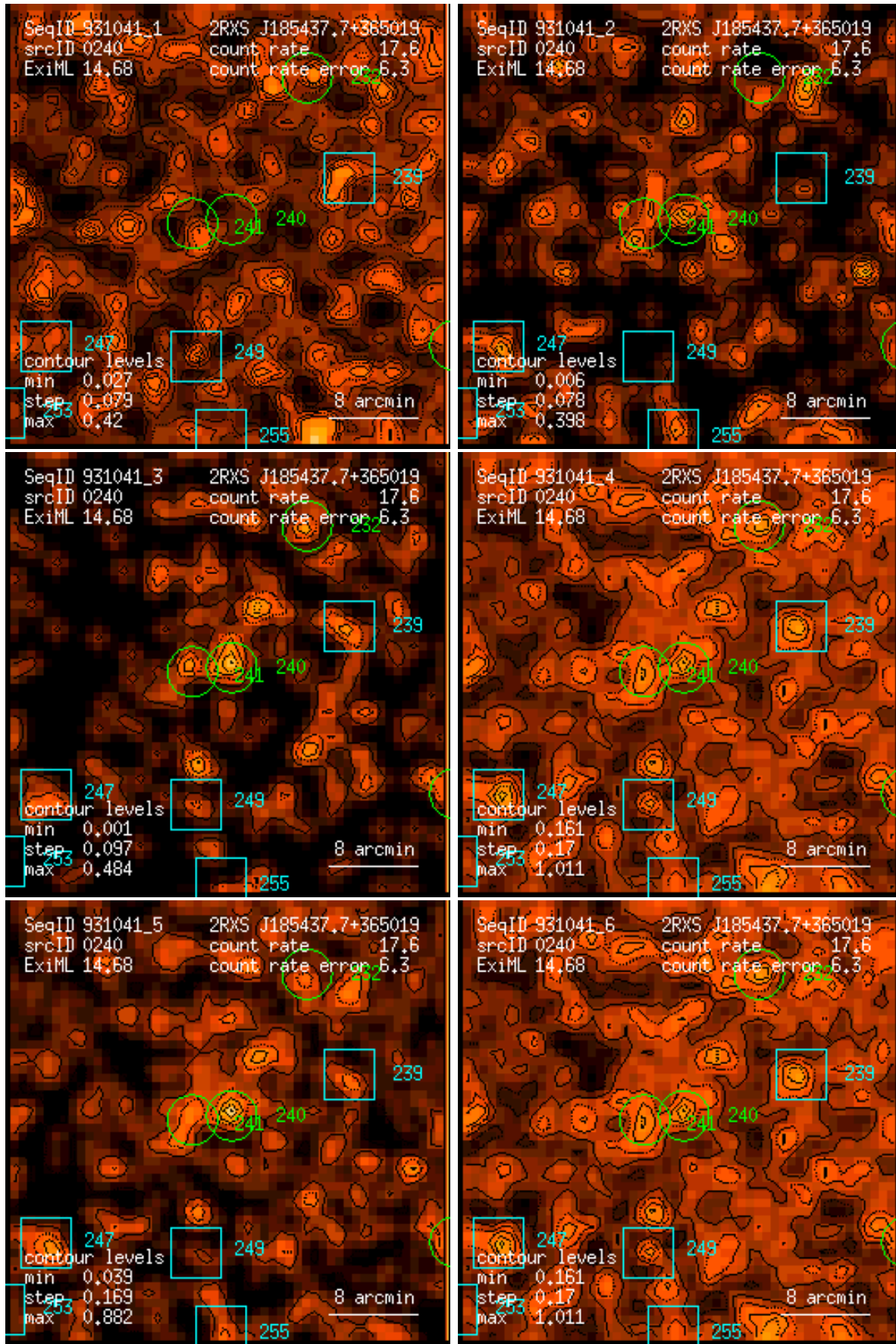
Figure 240: RASS 931041: detection 0240: band rate images, Gaussian filter: (1) PSPC channels 11 – 41, (2) 52 – 90, (3) 91 – 201, (4) 11 – 235, (5) 52 – 201, (6) 11 – 201. Broad band rates in counts/ks. Band rate contour levels in counts/ks/arcmin 2 .
