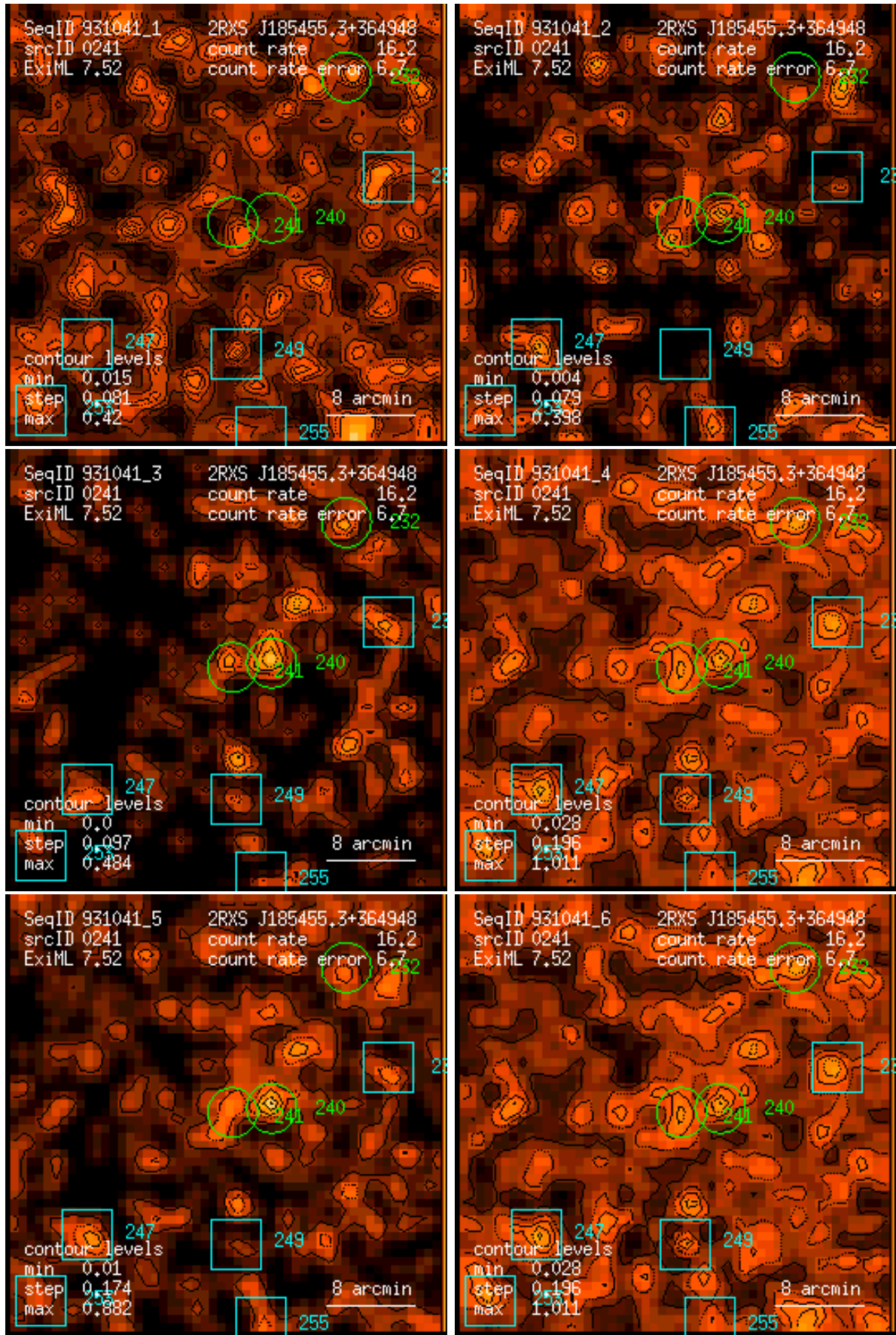
Figure 241: RASS 931041: detection 0241: band rate images, Gaussian filter: (1) PSPC channels 11 – 41, (2) 52 – 90, (3) 91 – 201, (4) 11 – 235, (5) 52 – 201, (6) 11 – 201. Broad band rates in counts/ks. Band rate contour levels in counts/ks/arcmin 2 .
