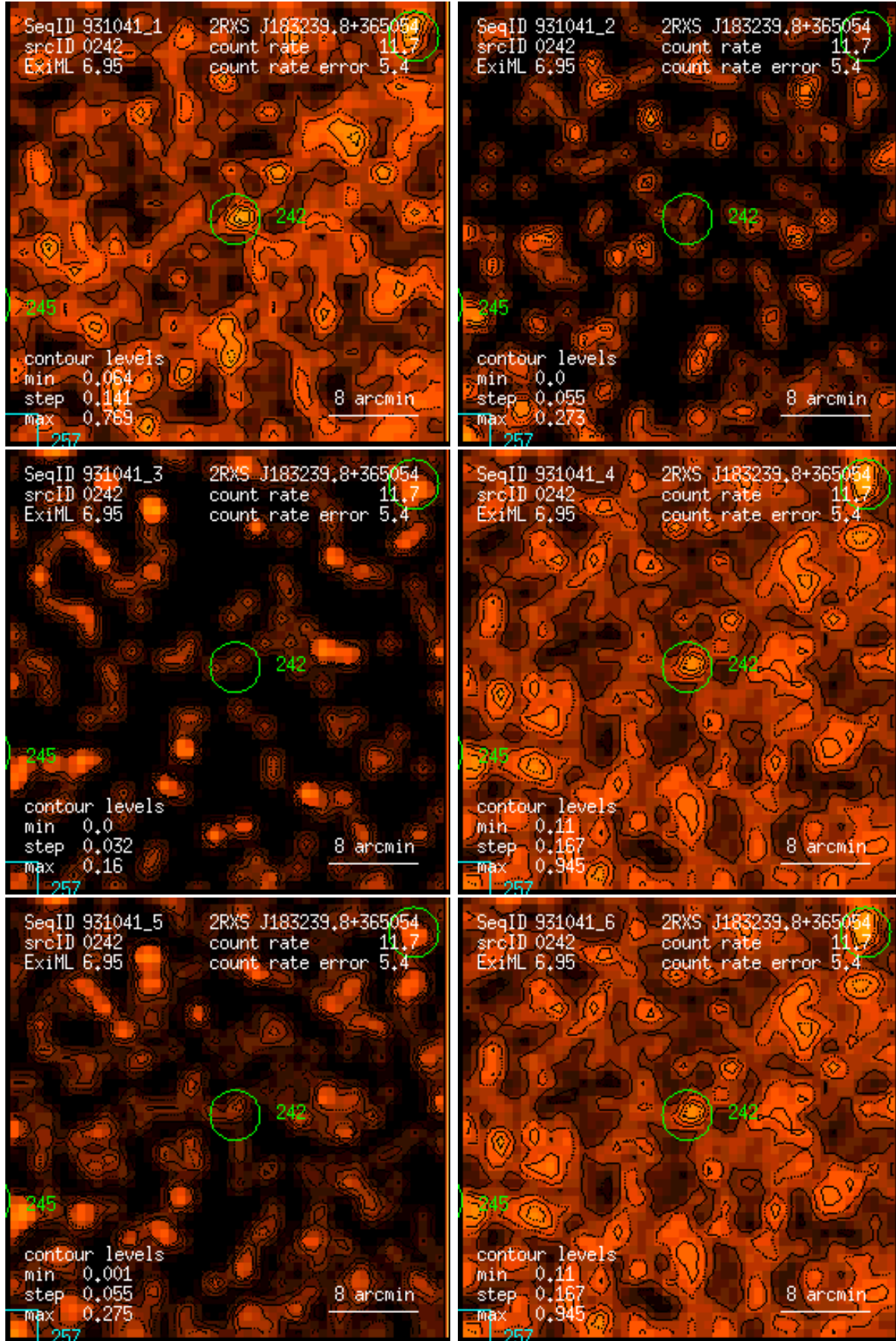
Figure 242: RASS 931041: detection 0242: band rate images, Gaussian filter: (1) PSPC channels 11 – 41, (2) 52 – 90, (3) 91 – 201, (4) 11 – 235, (5) 52 – 201, (6) 11 – 201. Broad band rates in counts/ks. Band rate contour levels in counts/ks/arcmin 2 .
