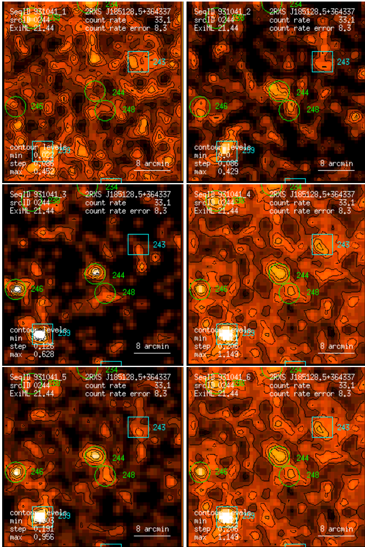
Figure 244: RASS 931041: detection 0244: band rate images, Gaussian filter: (1) PSPC channels 11 – 41, (2) 52 – 90, (3) 91 – 201, (4) 11 – 235, (5) 52 – 201, (6) 11 – 201. Broad band rates in counts/ks. Band rate contour levels in counts/ks/arcmin 2 .
