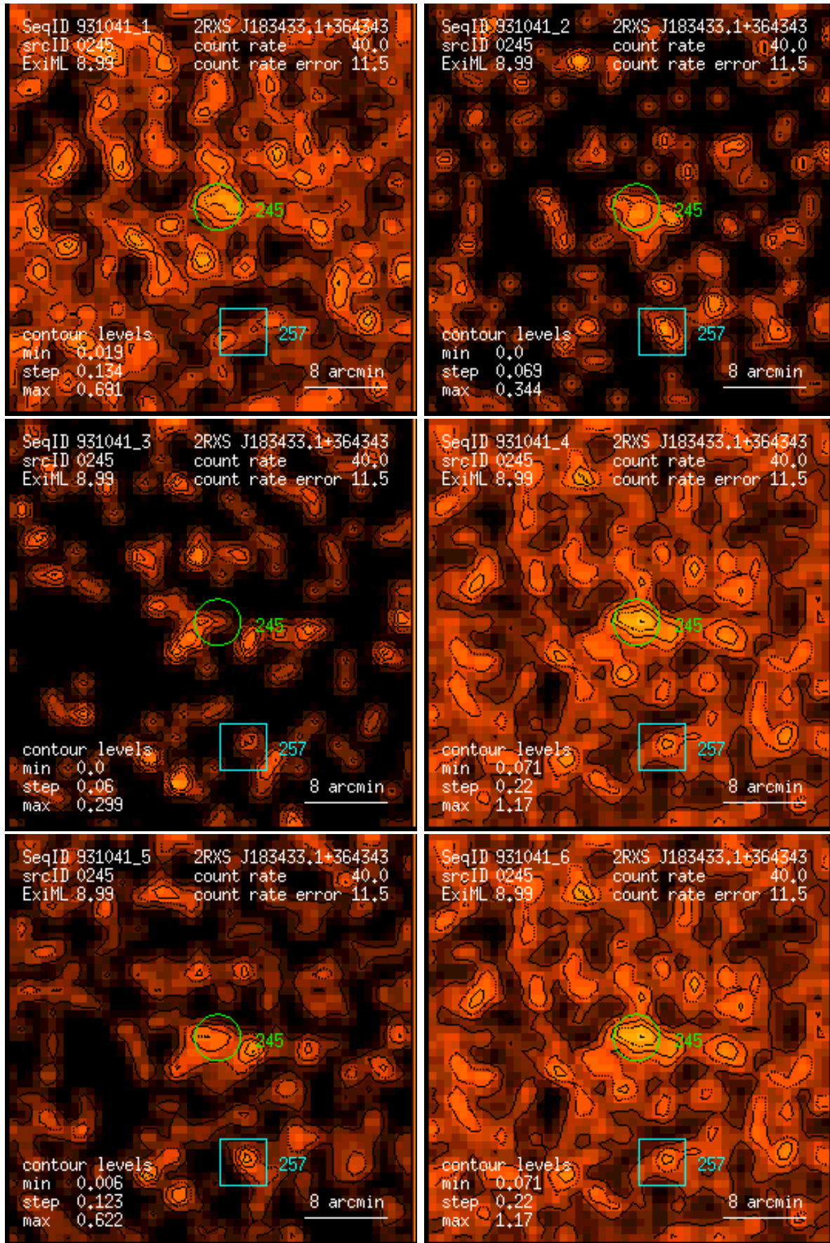
Figure 245: RASS 931041: detection 0245: band rate images, Gaussian filter: (1) PSPC channels 11 – 41, (2) 52 – 90, (3) 91 – 201, (4) 11 – 235, (5) 52 – 201, (6) 11 – 201. Broad band rates in counts/ks. Band rate contour levels in counts/ks/arcmin 2 .
