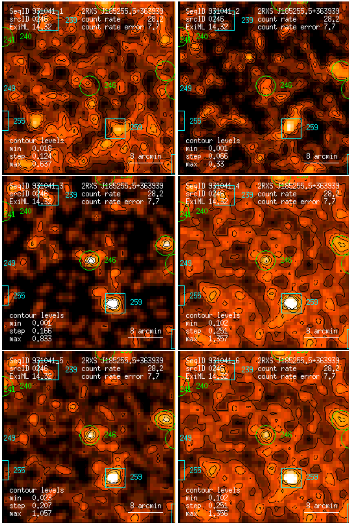
Figure 246: RASS 931041: detection 0246: band rate images, Gaussian filter: (1) PSPC channels 11 – 41, (2) 52 – 90, (3) 91 – 201, (4) 11 – 235, (5) 52 – 201, (6) 11 – 201. Broad band rates in counts/ks. Band rate contour levels in counts/ks/arcmin 2 .
