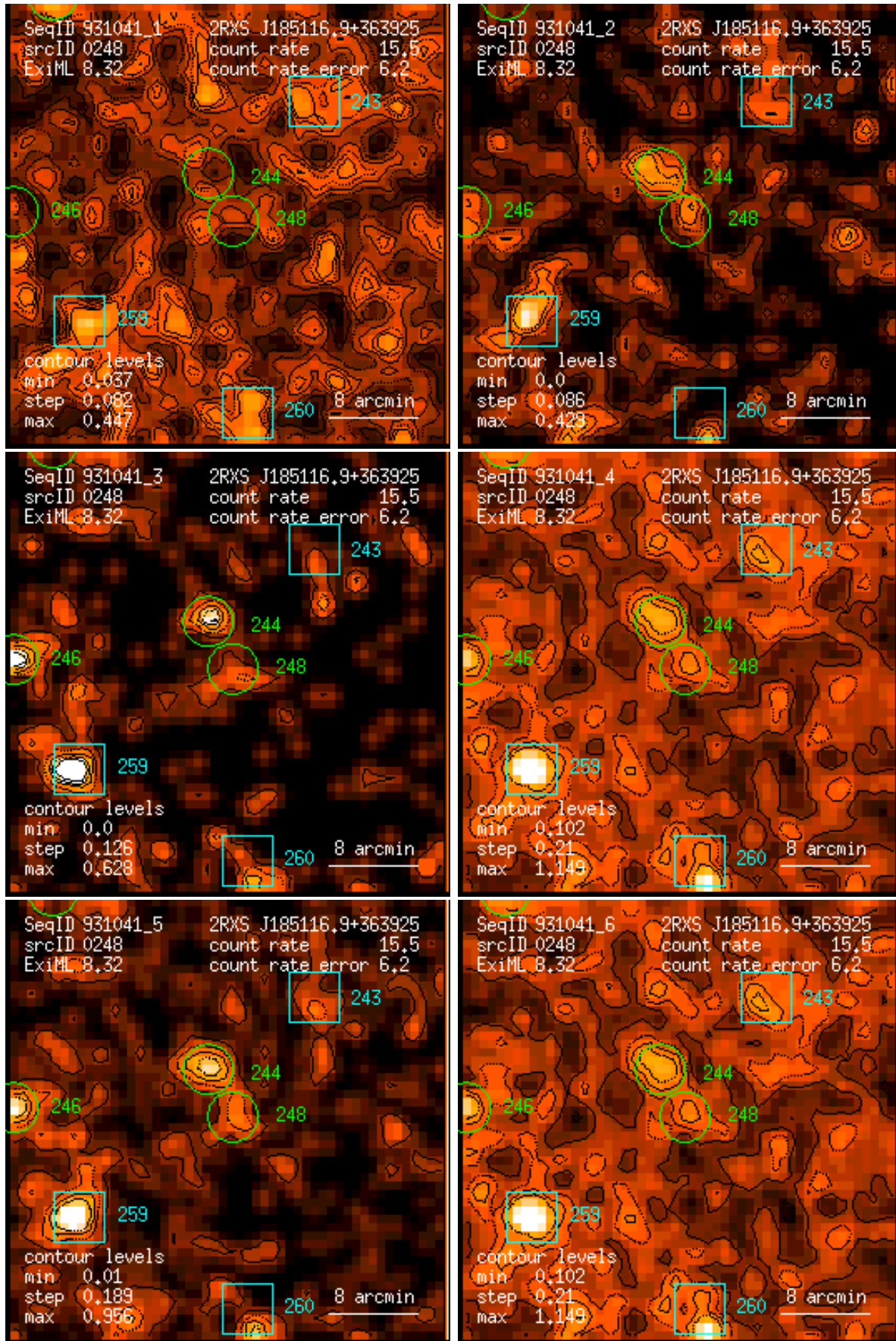
Figure 248: RASS 931041: detection 0248: band rate images, Gaussian filter: (1) PSPC channels 11 – 41, (2) 52 – 90, (3) 91 – 201, (4) 11 – 235, (5) 52 – 201, (6) 11 – 201. Broad band rates in counts/ks. Band rate contour levels in counts/ks/arcmin 2 .
