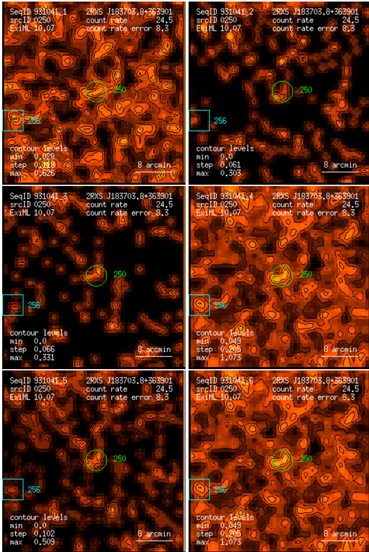
Figure 250: RASS 931041: detection 0250: band rate images, Gaussian filter: (1) PSPC channels 11 – 41, (2) 52 – 90, (3) 91 – 201, (4) 11 – 235, (5) 52 – 201, (6) 11 – 201. Broad band rates in counts/ks. Band rate contour levels in counts/ks/arcmin 2 .
