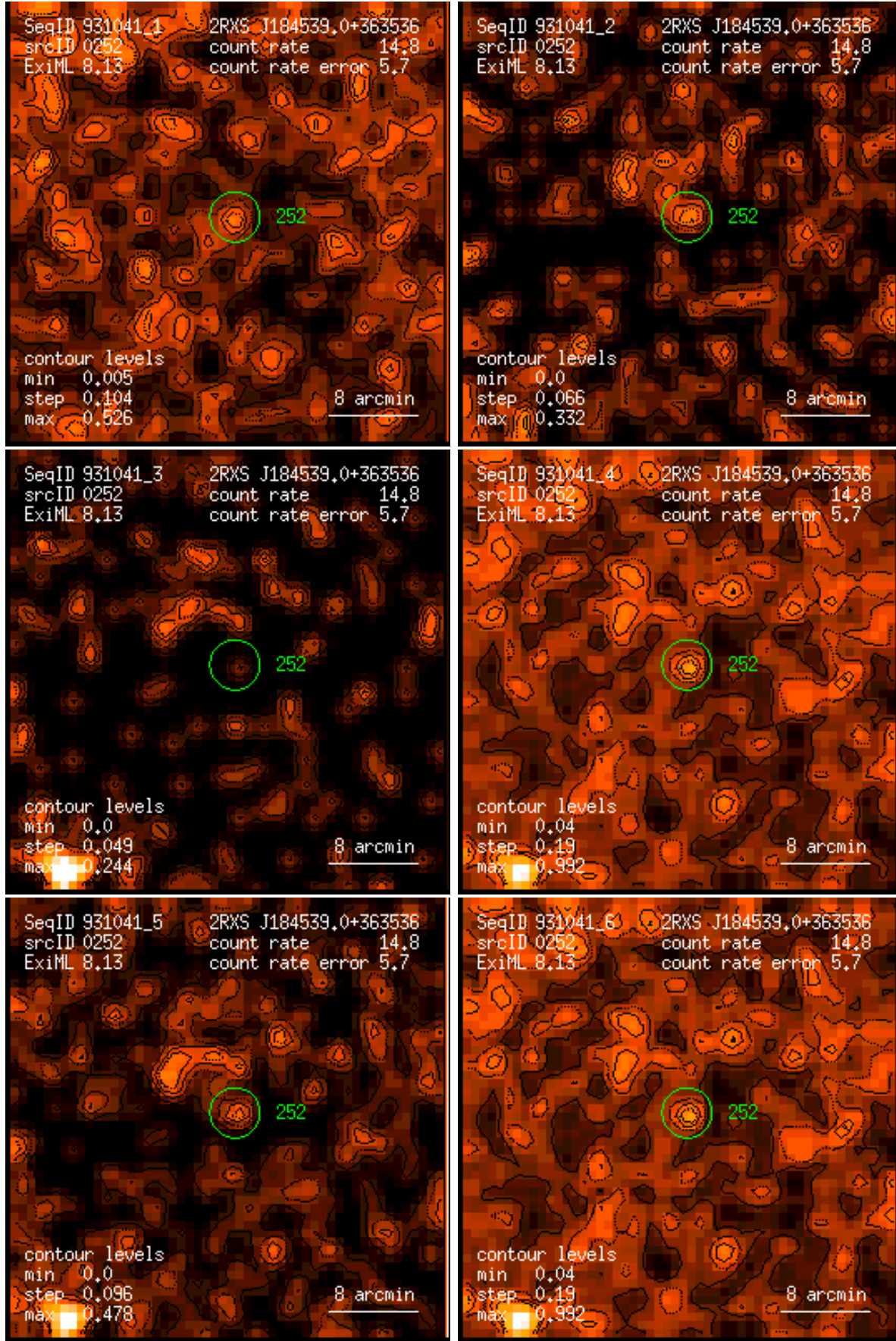
Figure 252: RASS 931041: detection 0252: band rate images, Gaussian filter: (1) PSPC channels 11 – 41, (2) 52 – 90, (3) 91 – 201, (4) 11 – 235, (5) 52 – 201, (6) 11 – 201. Broad band rates in counts/ks. Band rate contour levels in counts/ks/arcmin 2 .
