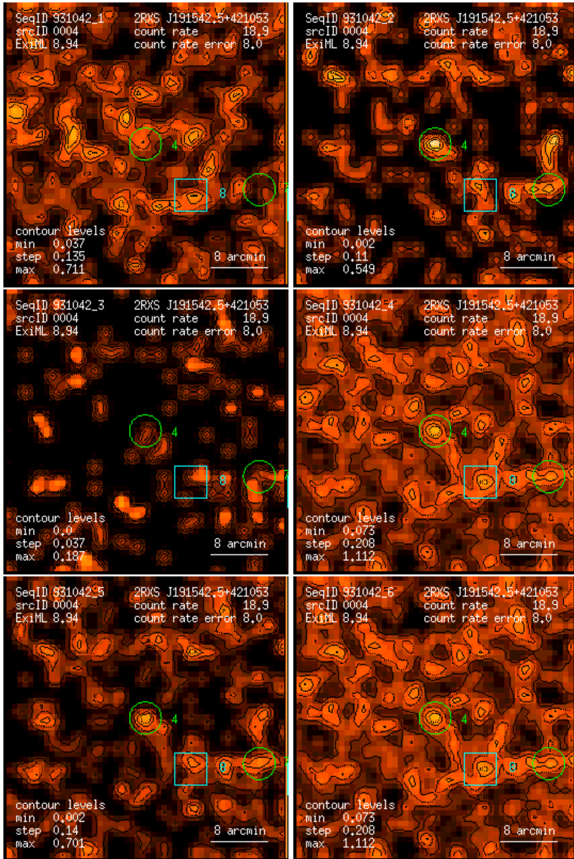
Figure 4: RASS 931042: detection 0004: band rate images, Gaussian filter: (1) PSPC channels 11 – 41, (2) 52 – 90, (3) 91 – 201, (4) 11 – 235, (5) 52 – 201, (6) 11 – 201. Broad band rates in counts/ks. Band rate contour levels in counts/ks/arcmin 2 .
