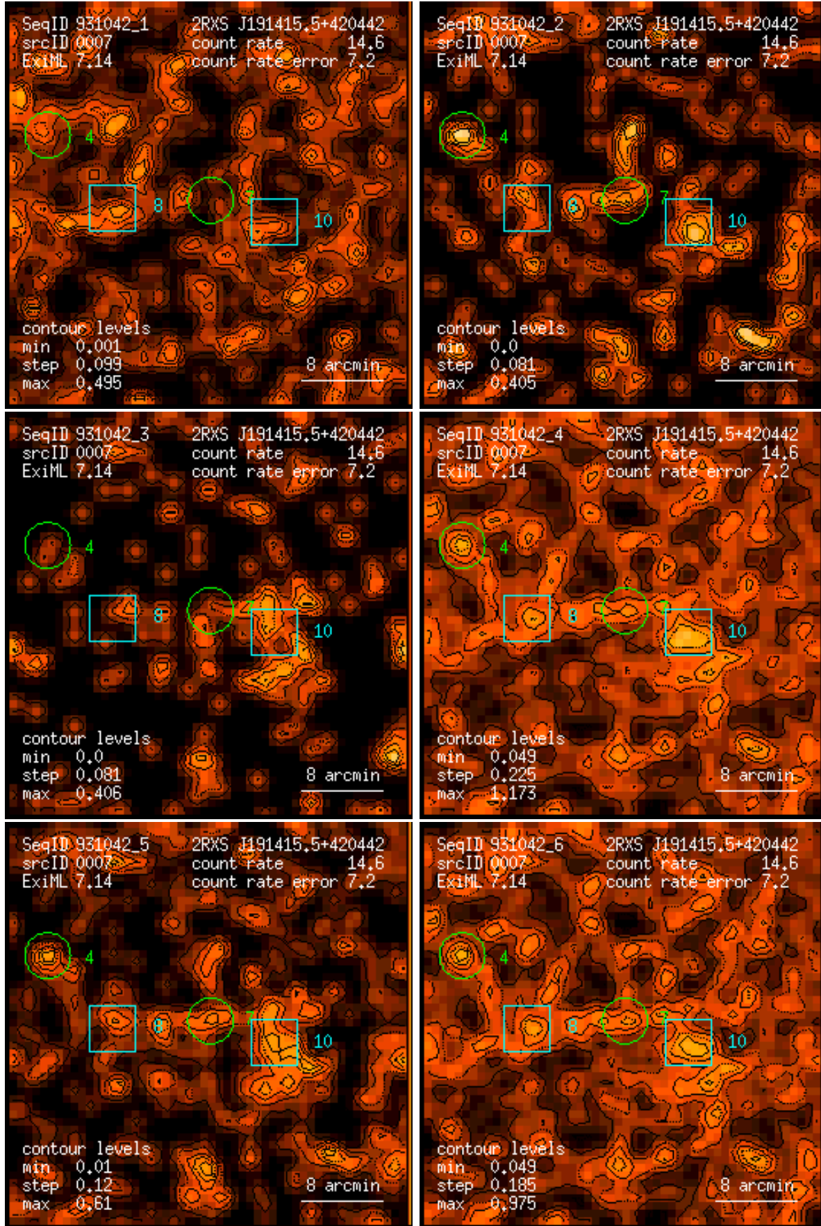
Figure 7: RASS 931042: detection 0007: band rate images, Gaussian filter: (1) PSPC channels 11 – 41, (2) 52 – 90, (3) 91 – 201, (4) 11 – 235, (5) 52 – 201, (6) 11 – 201. Broad band rates in counts/ks. Band rate contour levels in counts/ks/arcmin 2 .
