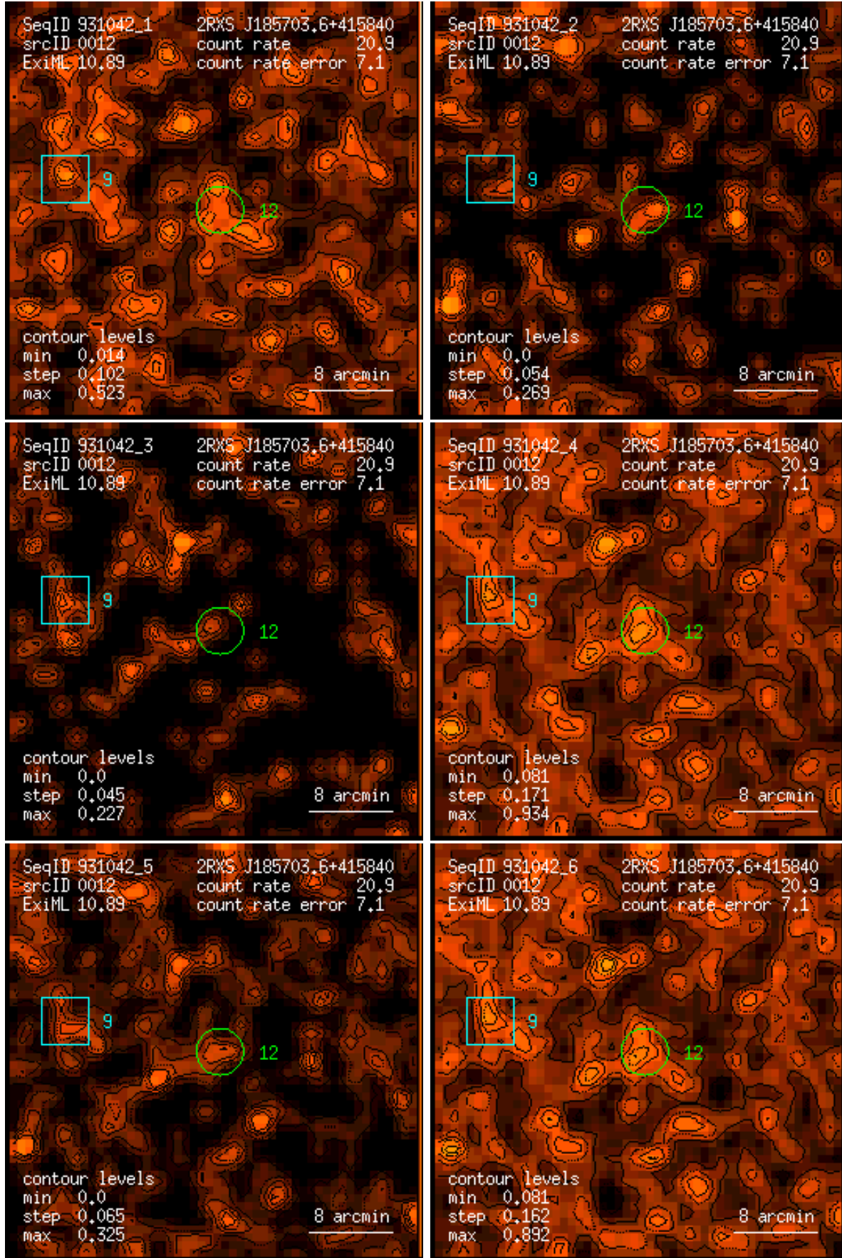
Figure 12: RASS 931042: detection 0012: band rate images, Gaussian filter: (1) PSPC channels 11 – 41, (2) 52 – 90, (3) 91 – 201, (4) 11 – 235, (5) 52 – 201, (6) 11 – 201. Broad band rates in counts/ks. Band rate contour levels in counts/ks/arcmin 2 .
