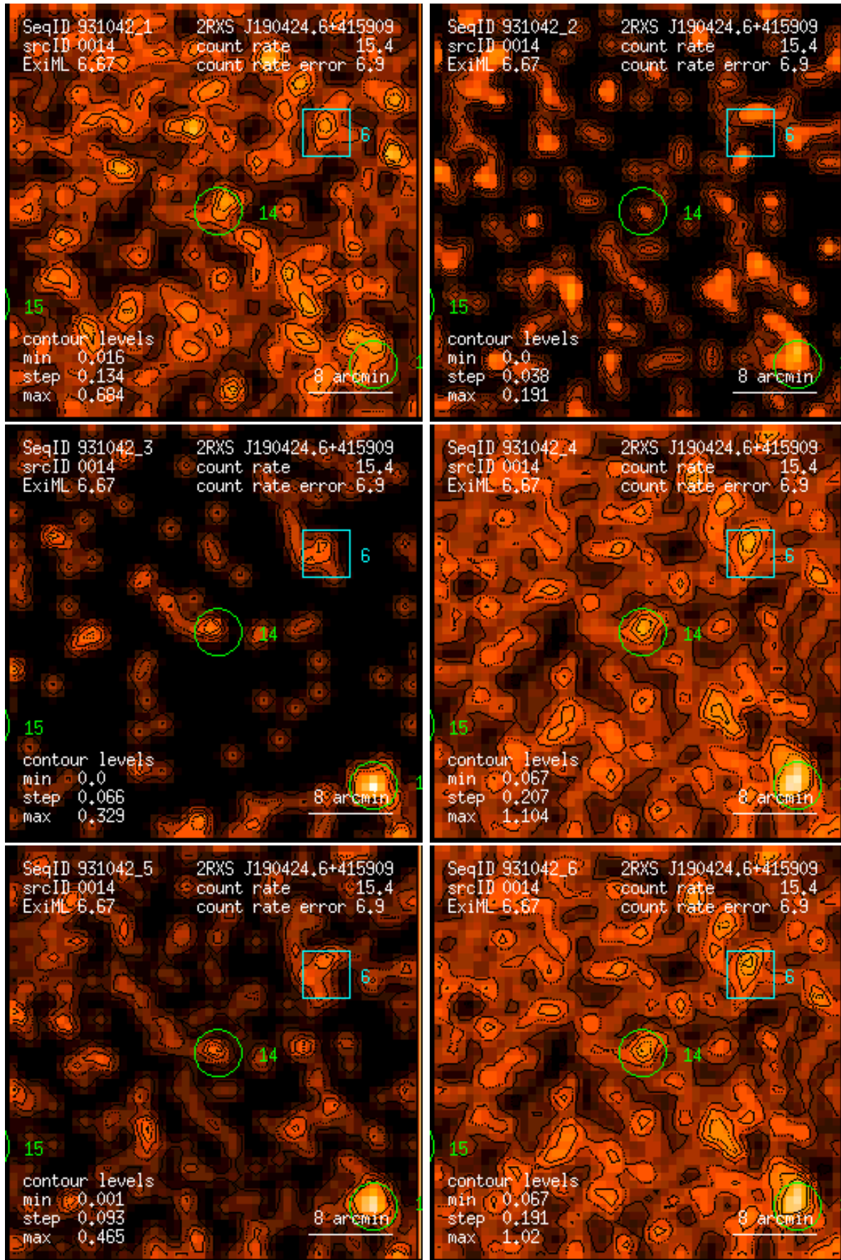
Figure 14: RASS 931042: detection 0014: band rate images, Gaussian filter: (1) PSPC channels 11 – 41, (2) 52 – 90, (3) 91 – 201, (4) 11 – 235, (5) 52 – 201, (6) 11 – 201. Broad band rates in counts/ks. Band rate contour levels in counts/ks/arcmin 2 .
