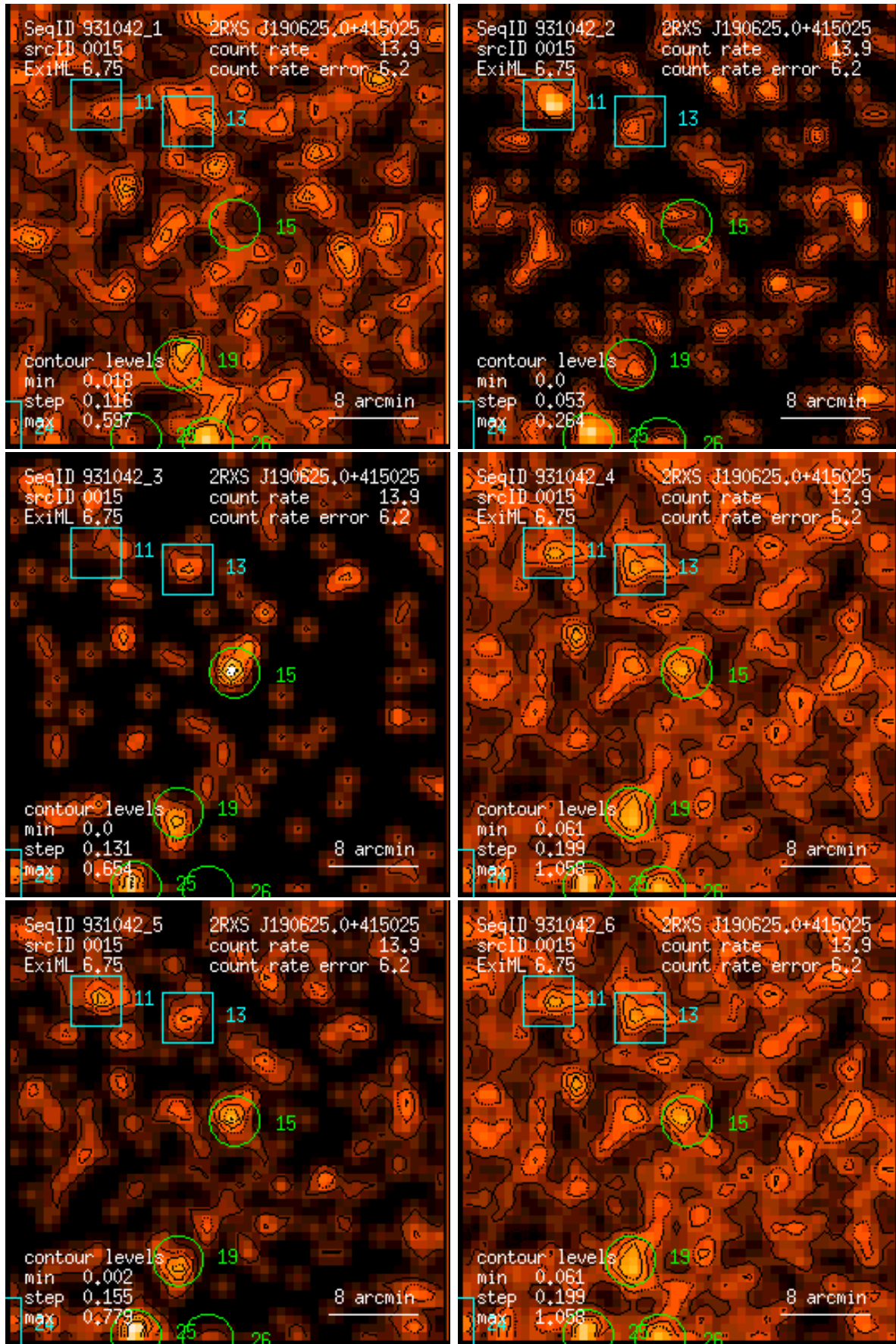
Figure 15: RASS 931042: detection 0015: band rate images, Gaussian filter: (1) PSPC channels 11 – 41, (2) 52 – 90, (3) 91 – 201, (4) 11 – 235, (5) 52 – 201, (6) 11 – 201. Broad band rates in counts/ks. Band rate contour levels in counts/ks/arcmin 2 .
