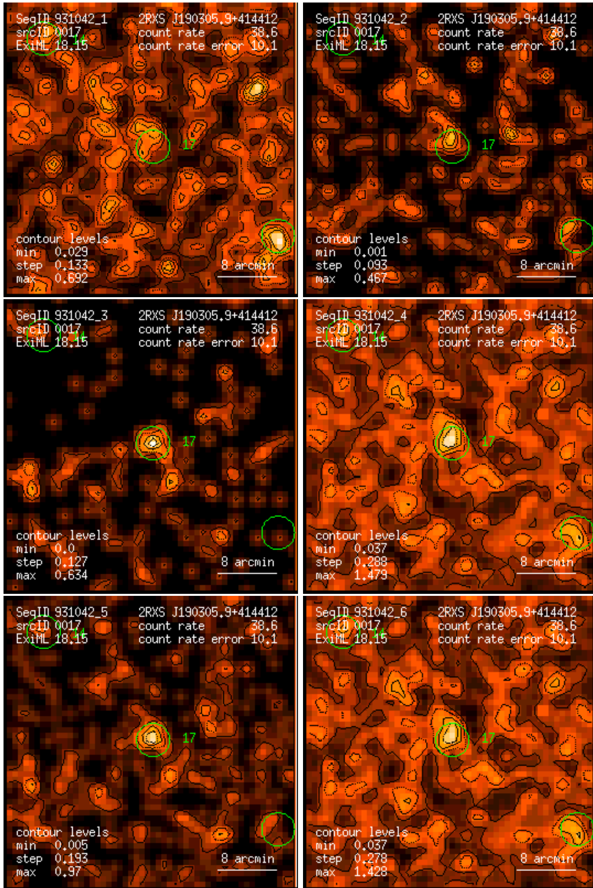
Figure 17: RASS 931042: detection 0017: band rate images, Gaussian filter: (1) PSPC channels 11 – 41, (2) 52 – 90, (3) 91 – 201, (4) 11 – 235, (5) 52 – 201, (6) 11 – 201. Broad band rates in counts/ks. Band rate contour levels in counts/ks/arcmin 2 .
