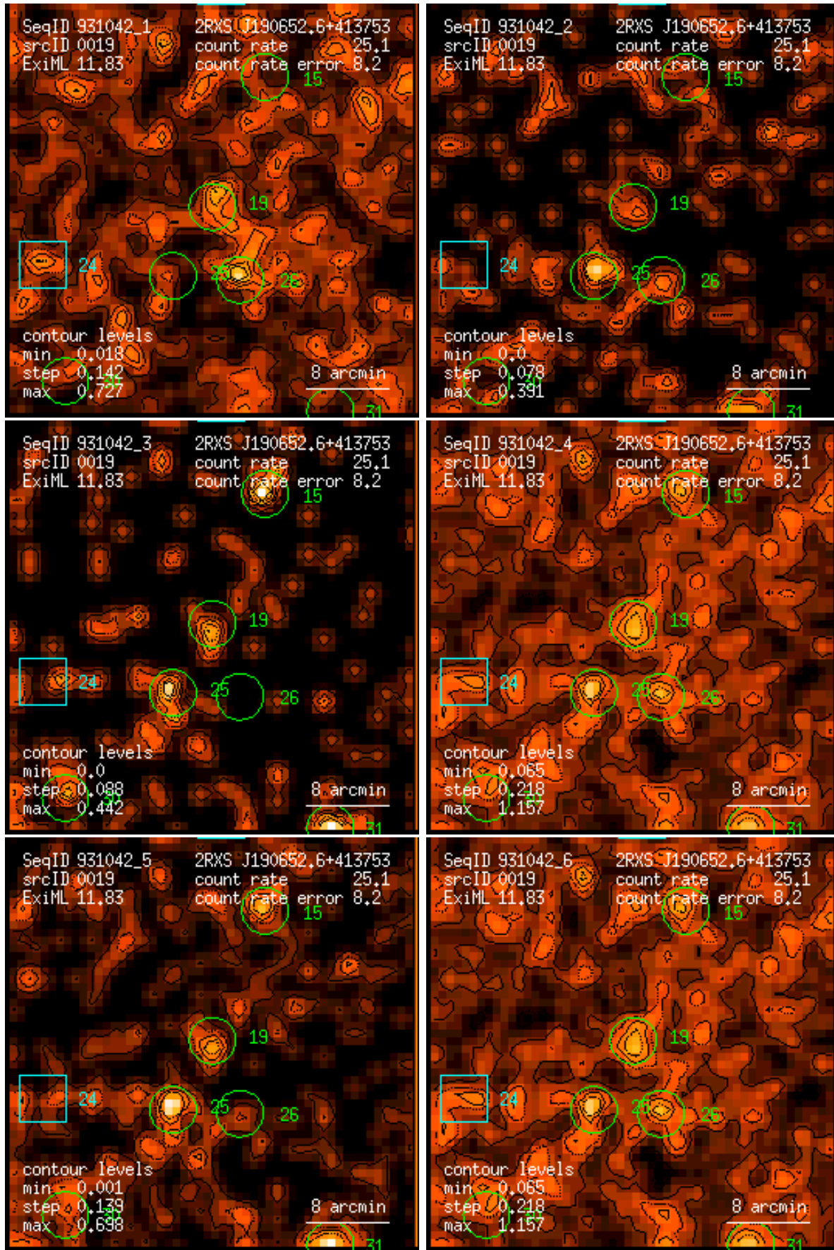
Figure 19: RASS 931042: detection 0019: band rate images, Gaussian filter: (1) PSPC channels 11 – 41, (2) 52 – 90, (3) 91 – 201, (4) 11 – 235, (5) 52 – 201, (6) 11 – 201. Broad band rates in counts/ks. Band rate contour levels in counts/ks/arcmin 2 .
