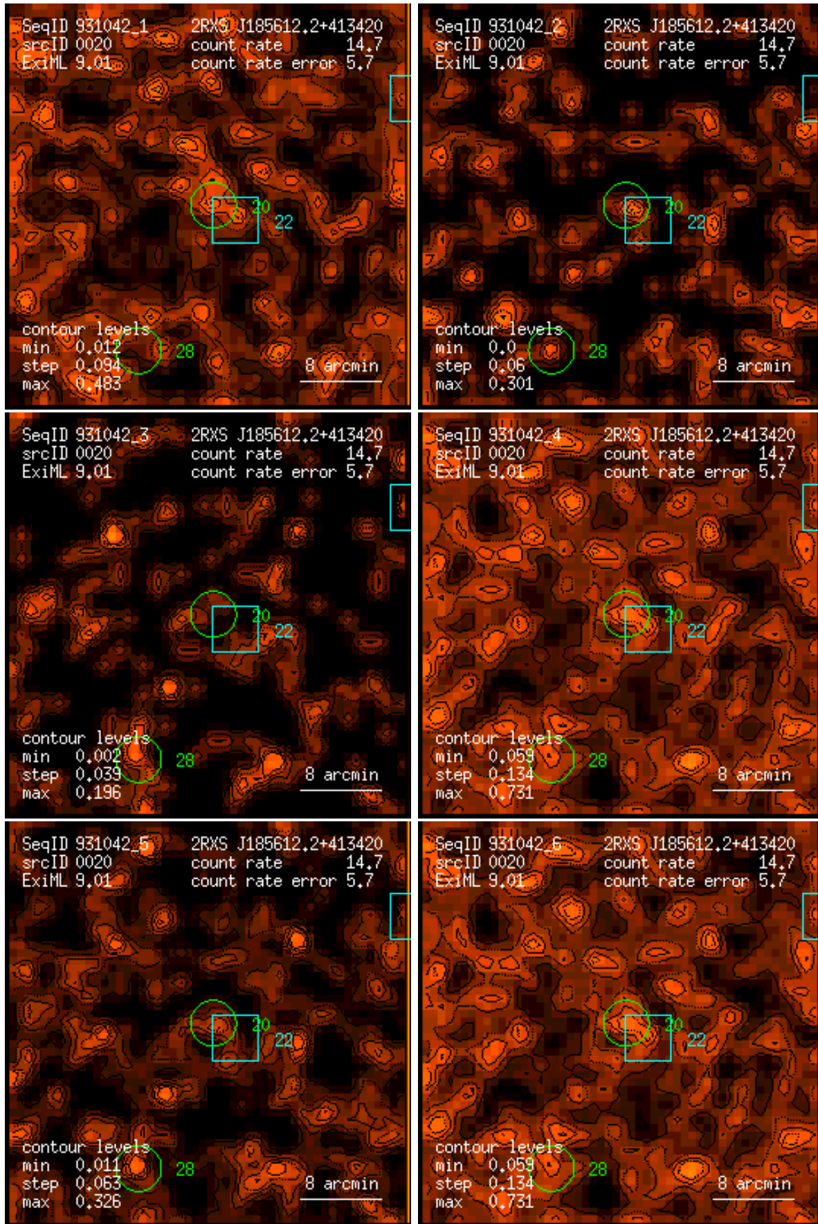
Figure 20: RASS 931042: detection 0020: band rate images, Gaussian filter: (1) PSPC channels 11 – 41, (2) 52 – 90, (3) 91 – 201, (4) 11 – 235, (5) 52 – 201, (6) 11 – 201. Broad band rates in counts/ks. Band rate contour levels in counts/ks/arcmin 2 .
