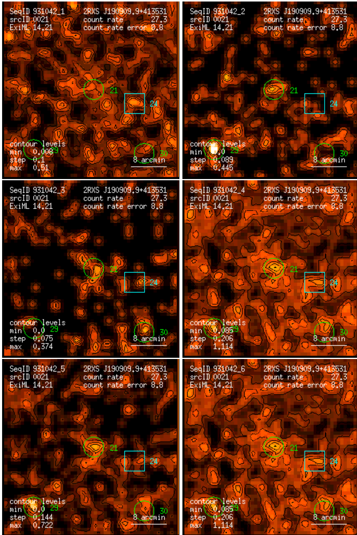
Figure 21: RASS 931042: detection 0021: band rate images, Gaussian filter: (1) PSPC channels 11 – 41, (2) 52 – 90, (3) 91 – 201, (4) 11 – 235, (5) 52 – 201, (6) 11 – 201. Broad band rates in counts/ks. Band rate contour levels in counts/ks/arcmin 2 .
