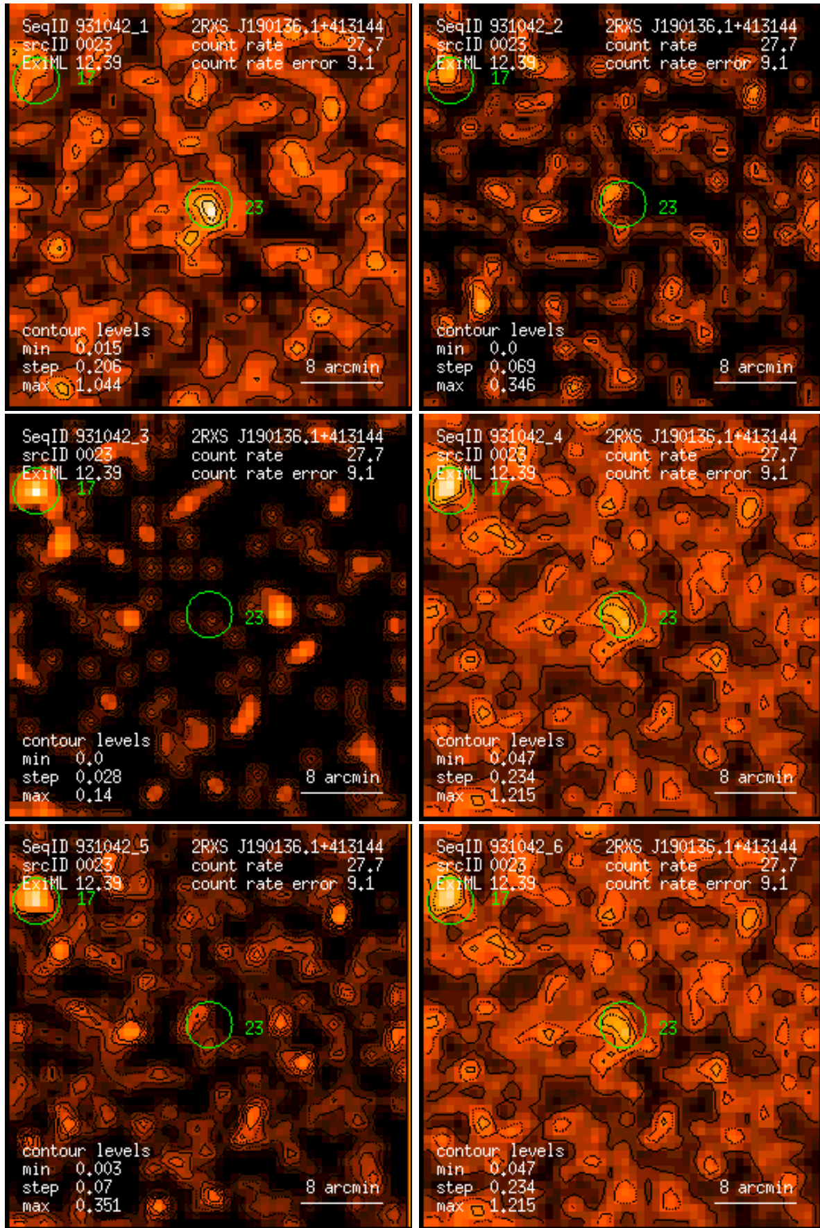
Figure 23: RASS 931042: detection 0023: band rate images, Gaussian filter: (1) PSPC channels 11 – 41, (2) 52 – 90, (3) 91 – 201, (4) 11 – 235, (5) 52 – 201, (6) 11 – 201. Broad band rates in counts/ks. Band rate contour levels in counts/ks/arcmin 2 .
