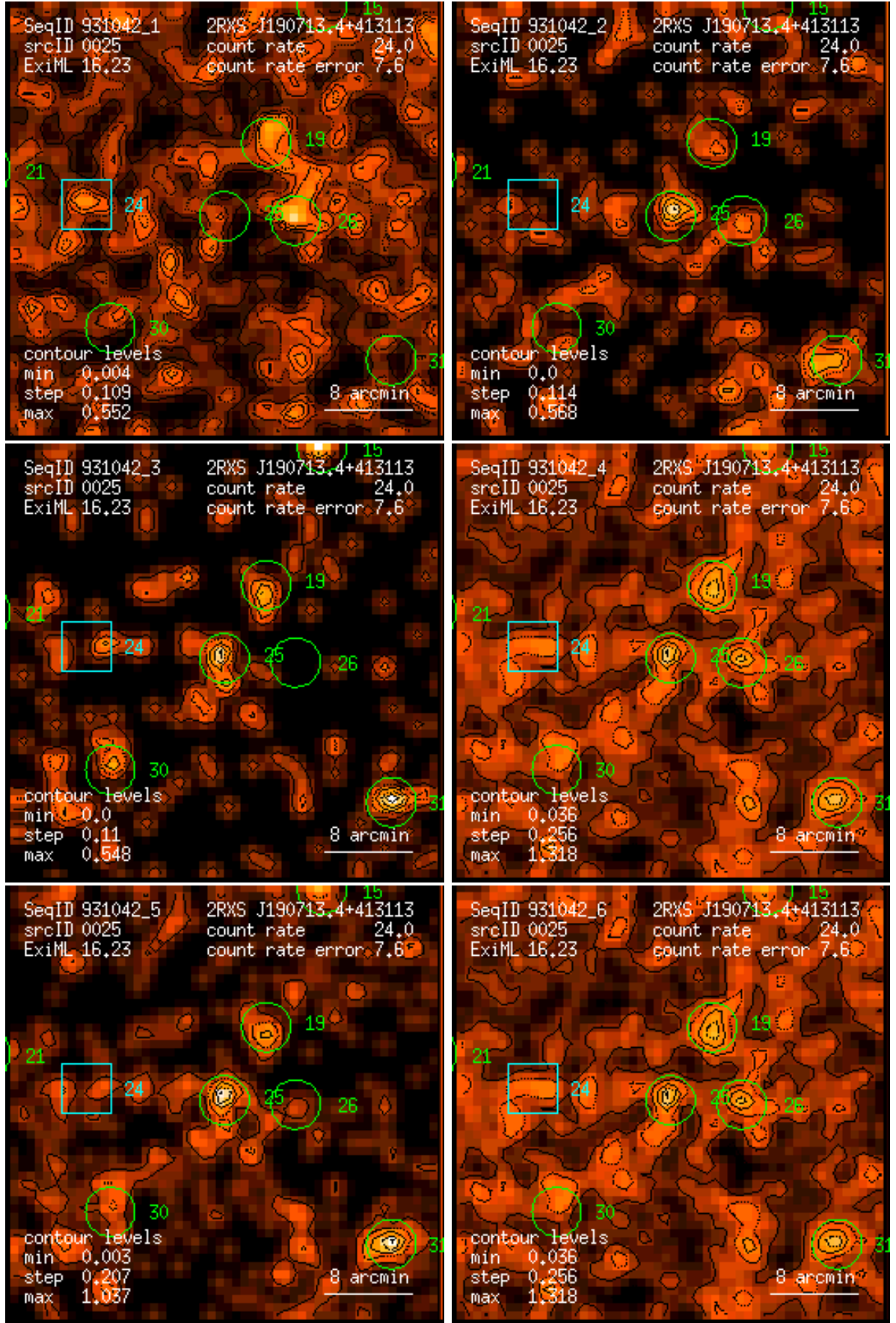
Figure 25: RASS 931042: detection 0025: band rate images, Gaussian filter: (1) PSPC channels 11 – 41, (2) 52 – 90, (3) 91 – 201, (4) 11 – 235, (5) 52 – 201, (6) 11 – 201. Broad band rates in counts/ks. Band rate contour levels in counts/ks/arcmin 2 .
