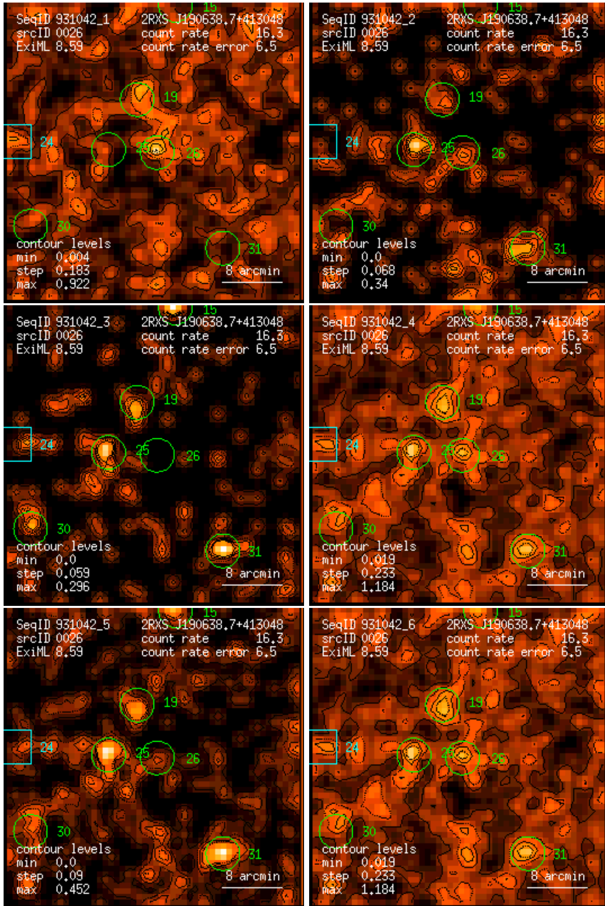
Figure 26: RASS 931042: detection 0026: band rate images, Gaussian filter: (1) PSPC channels 11 – 41, (2) 52 – 90, (3) 91 – 201, (4) 11 – 235, (5) 52 – 201, (6) 11 – 201. Broad band rates in counts/ks. Band rate contour levels in counts/ks/arcmin 2 .
