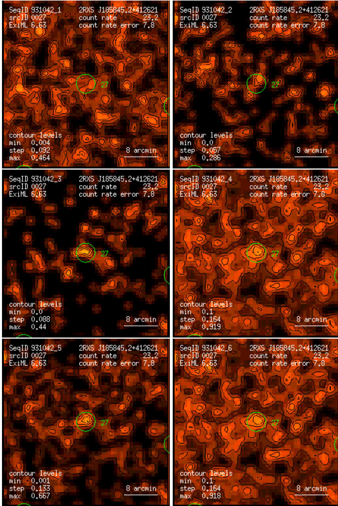
Figure 27: RASS 931042: detection 0027: band rate images, Gaussian filter: (1) PSPC channels 11 – 41, (2) 52 – 90, (3) 91 – 201, (4) 11 – 235, (5) 52 – 201, (6) 11 – 201. Broad band rates in counts/ks. Band rate contour levels in counts/ks/arcmin 2 .
