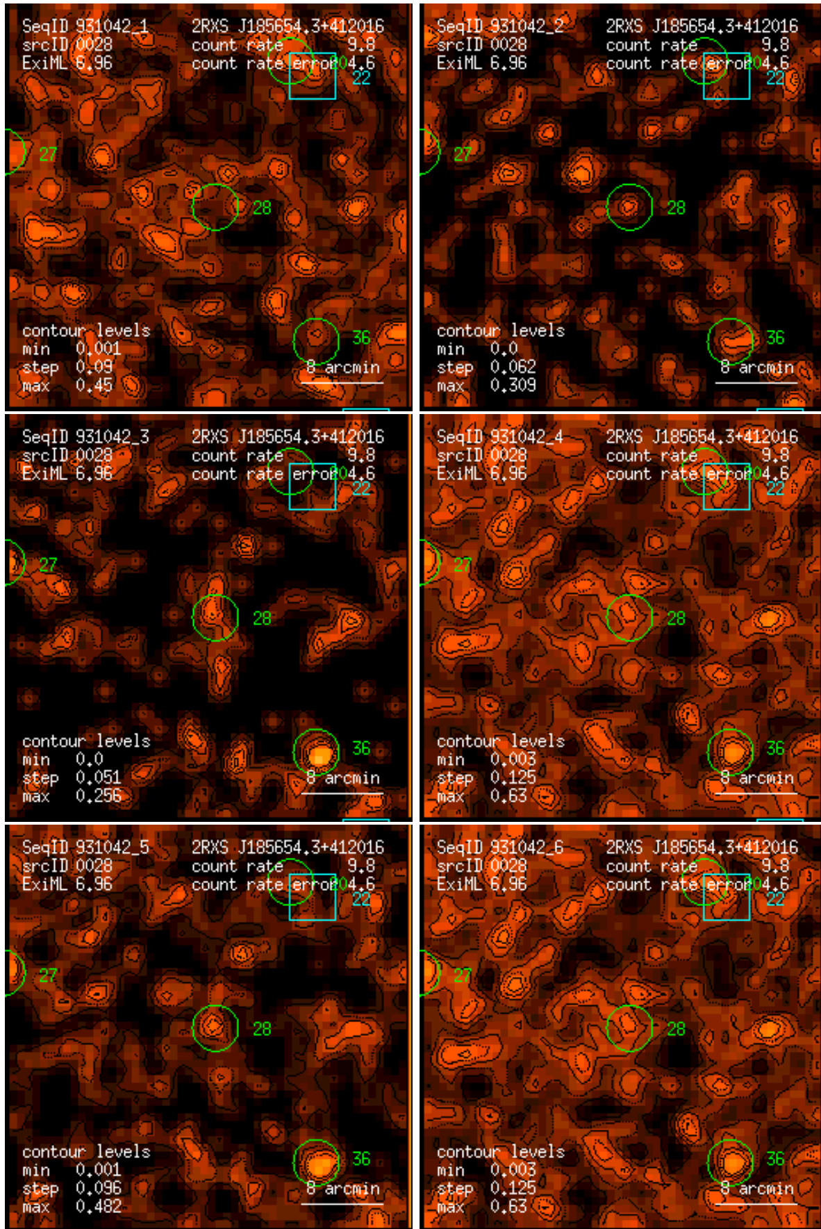
Figure 28: RASS 931042: detection 0028: band rate images, Gaussian filter: (1) PSPC channels 11 – 41, (2) 52 – 90, (3) 91 – 201, (4) 11 – 235, (5) 52 – 201, (6) 11 – 201. Broad band rates in counts/ks. Band rate contour levels in counts/ks/arcmin 2 .
