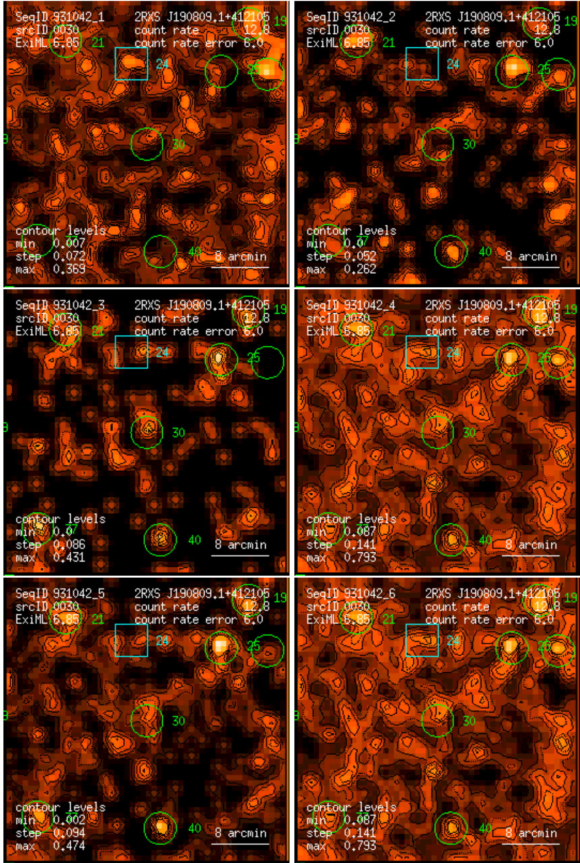
Figure 30: RASS 931042: detection 0030: band rate images, Gaussian filter: (1) PSPC channels 11 – 41, (2) 52 – 90, (3) 91 – 201, (4) 11 – 235, (5) 52 – 201, (6) 11 – 201. Broad band rates in counts/ks. Band rate contour levels in counts/ks/arcmin 2 .
