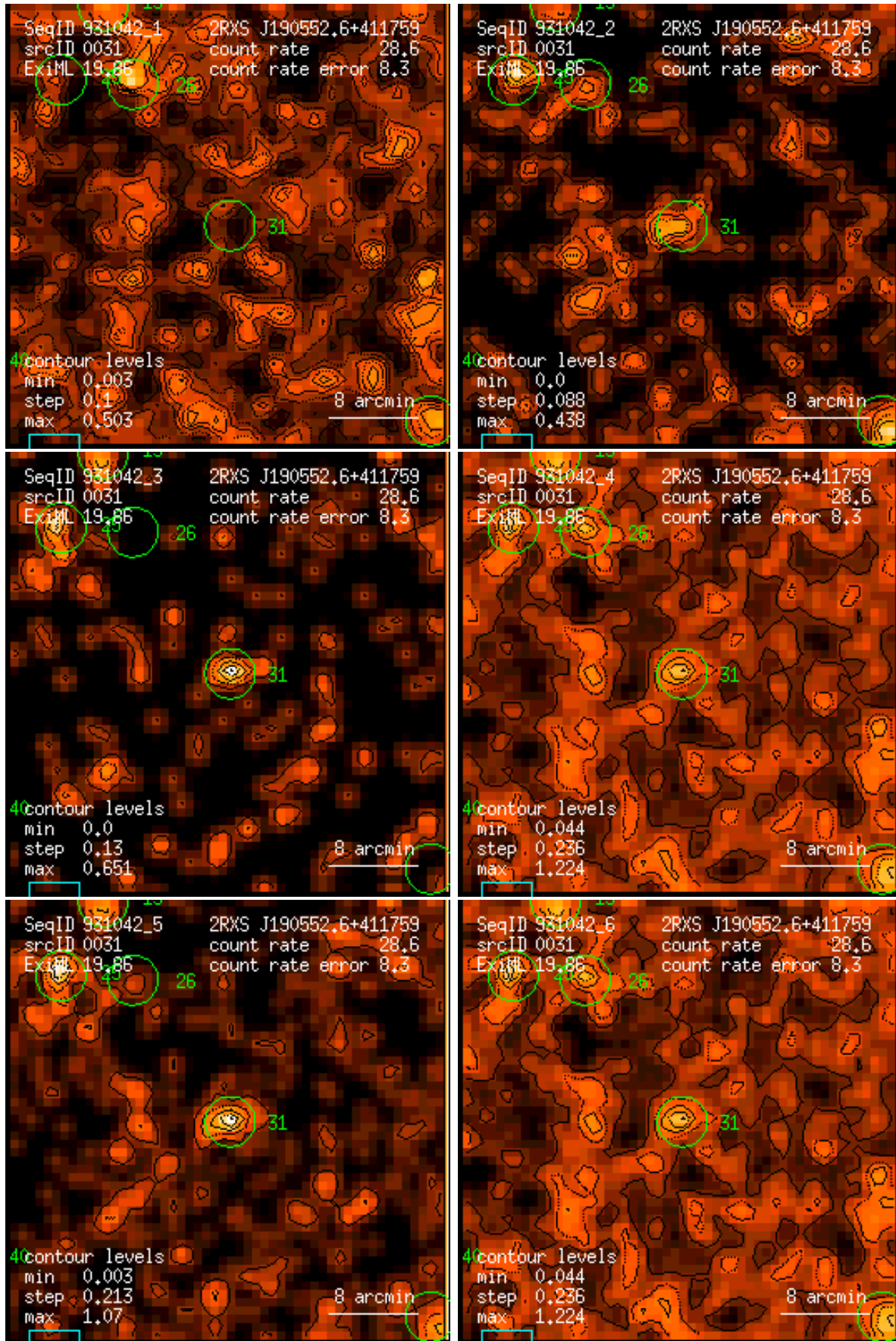
Figure 31: RASS 931042: detection 0031: band rate images, Gaussian filter: (1) PSPC channels 11 – 41, (2) 52 – 90, (3) 91 – 201, (4) 11 – 235, (5) 52 – 201, (6) 11 – 201. Broad band rates in counts/ks. Band rate contour levels in counts/ks/arcmin 2 .
