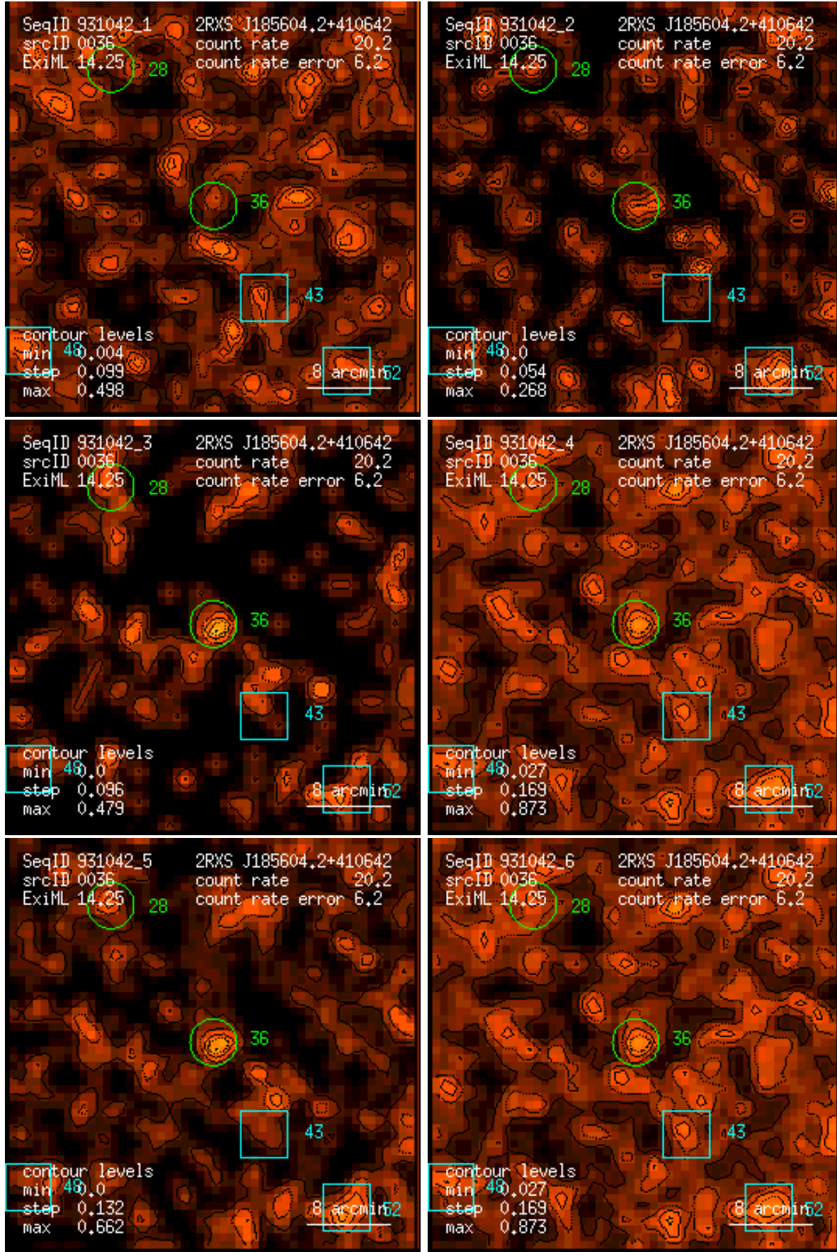
Figure 36: RASS 931042: detection 0036: band rate images, Gaussian filter: (1) PSPC channels 11 – 41, (2) 52 – 90, (3) 91 – 201, (4) 11 – 235, (5) 52 – 201, (6) 11 – 201. Broad band rates in counts/ks. Band rate contour levels in counts/ks/arcmin 2 .
