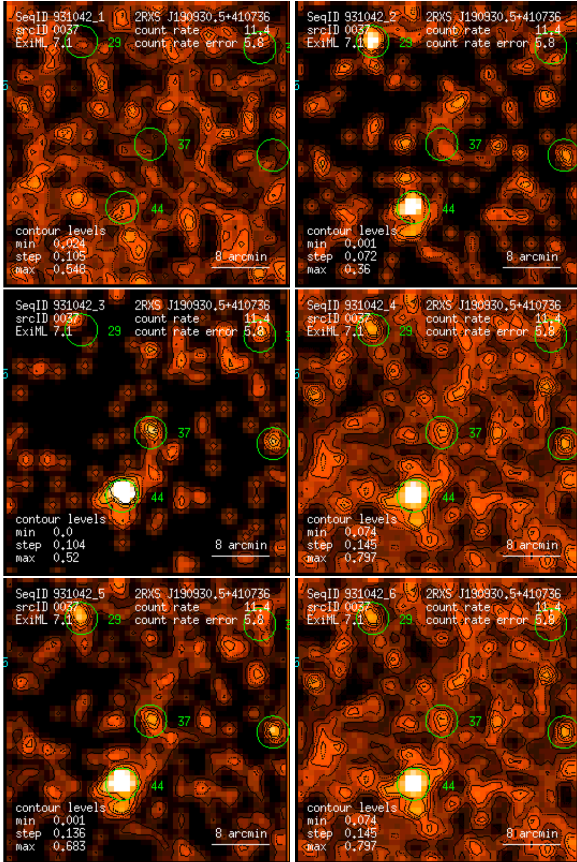
Figure 37: RASS 931042: detection 0037: band rate images, Gaussian filter: (1) PSPC channels 11 – 41, (2) 52 – 90, (3) 91 – 201, (4) 11 – 235, (5) 52 – 201, (6) 11 – 201. Broad band rates in counts/ks. Band rate contour levels in counts/ks/arcmin 2 .
