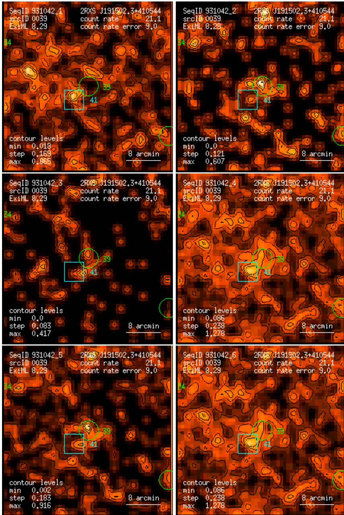
Figure 39: RASS 931042: detection 0039: band rate images, Gaussian filter: (1) PSPC channels 11 – 41, (2) 52 – 90, (3) 91 – 201, (4) 11 – 235, (5) 52 – 201, (6) 11 – 201. Broad band rates in counts/ks. Band rate contour levels in counts/ks/arcmin 2 .
