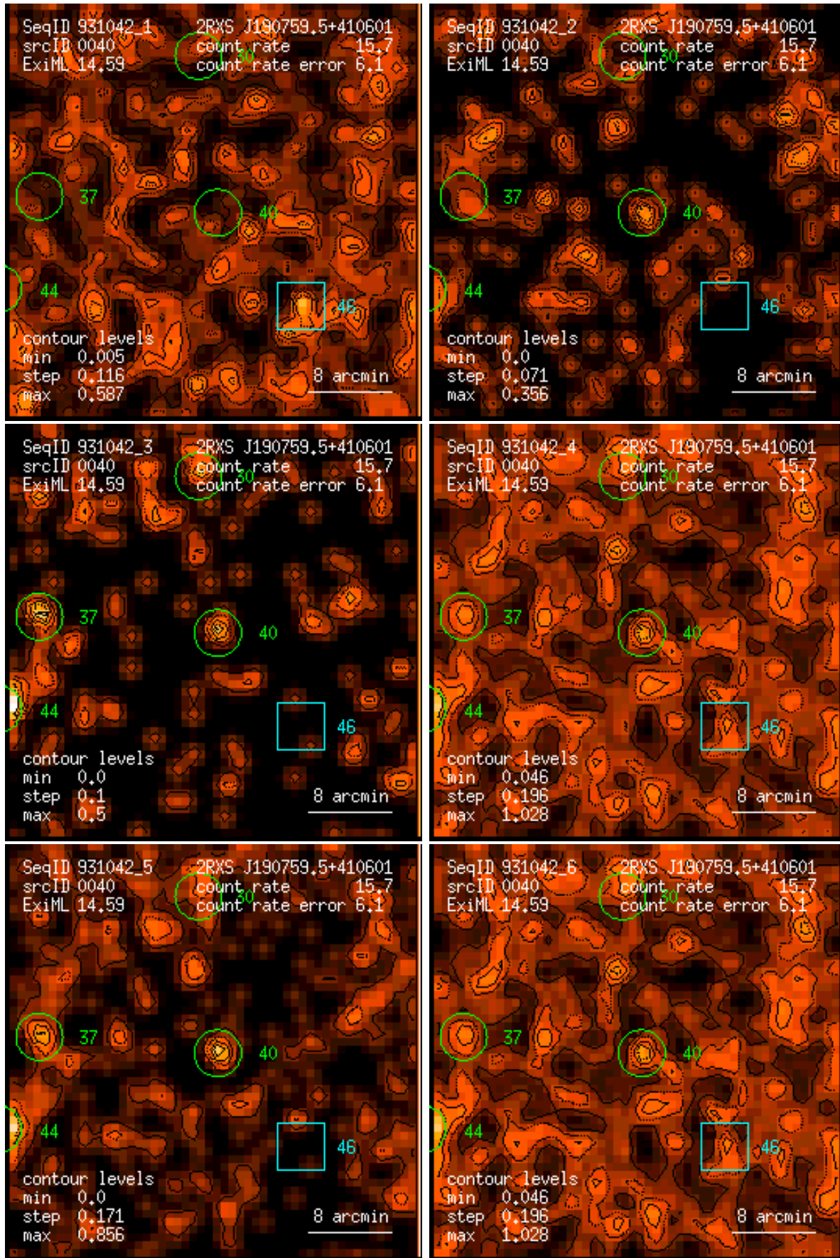
Figure 40: RASS 931042: detection 0040: band rate images, Gaussian filter: (1) PSPC channels 11 – 41, (2) 52 – 90, (3) 91 – 201, (4) 11 – 235, (5) 52 – 201, (6) 11 – 201. Broad band rates in counts/ks. Band rate contour levels in counts/ks/arcmin 2 .
