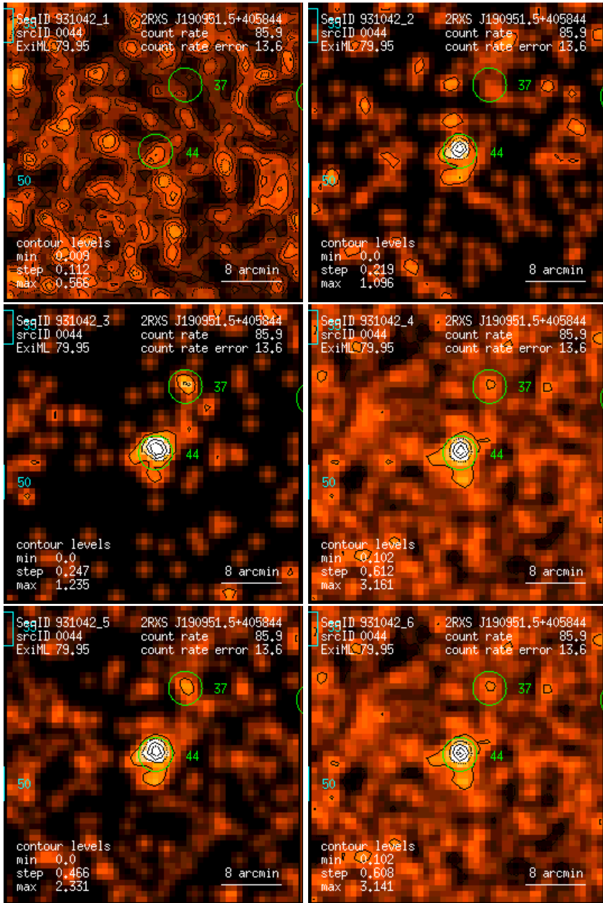
Figure 44: RASS 931042: detection 0044: band rate images, Gaussian filter: (1) PSPC channels 11 – 41, (2) 52 – 90, (3) 91 – 201, (4) 11 – 235, (5) 52 – 201, (6) 11 – 201. Broad band rates in counts/ks. Band rate contour levels in counts/ks/arcmin 2 .
