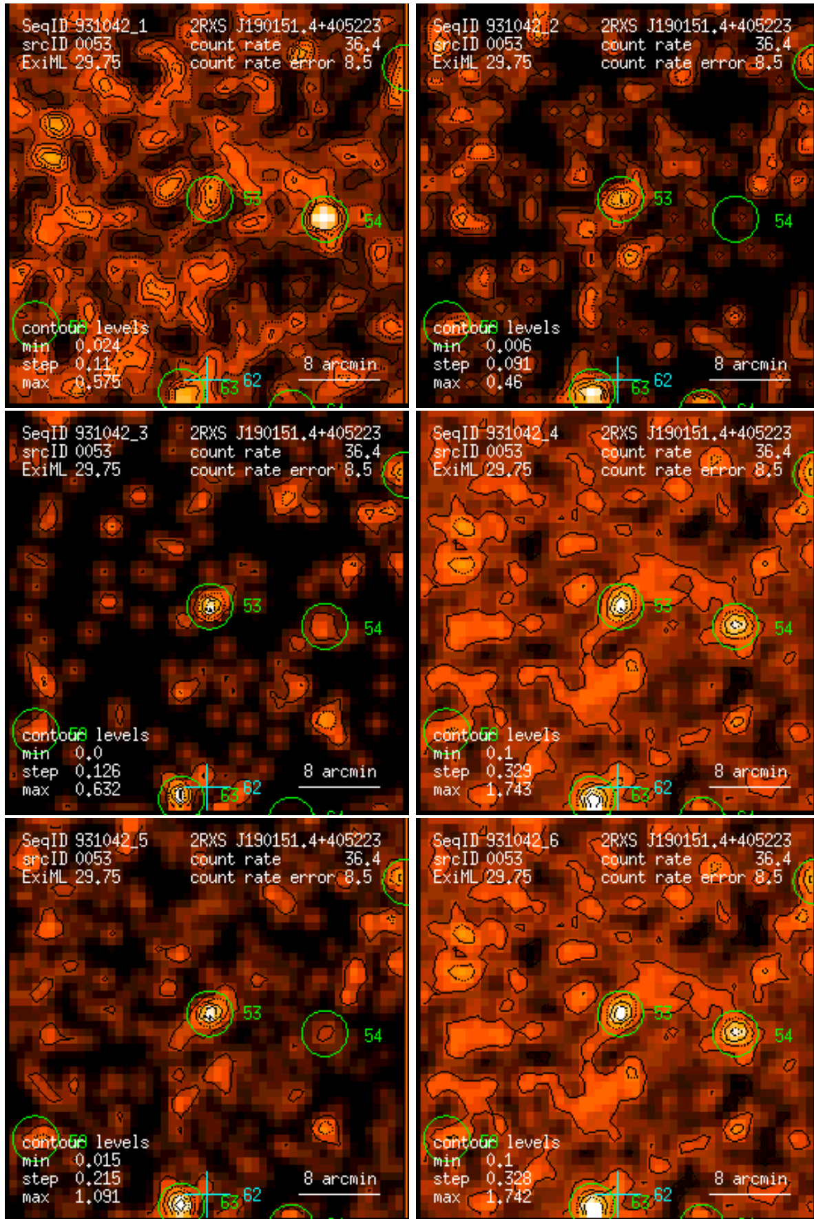
Figure 53: RASS 931042: detection 0053: band rate images, Gaussian filter: (1) PSPC channels 11 – 41, (2) 52 – 90, (3) 91 – 201, (4) 11 – 235, (5) 52 – 201, (6) 11 – 201. Broad band rates in counts/ks. Band rate contour levels in counts/ks/arcmin 2 .
