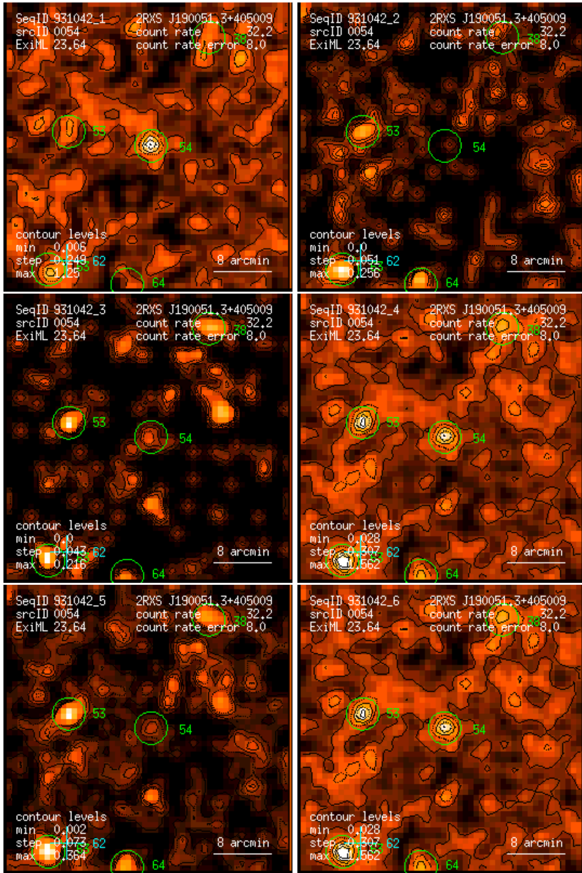
Figure 54: RASS 931042: detection 0054: band rate images, Gaussian filter: (1) PSPC channels 11 – 41, (2) 52 – 90, (3) 91 – 201, (4) 11 – 235, (5) 52 – 201, (6) 11 – 201. Broad band rates in counts/ks. Band rate contour levels in counts/ks/arcmin 2 .
