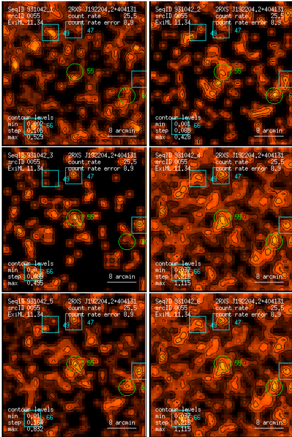
Figure 55: RASS 931042: detection 0055: band rate images, Gaussian filter: (1) PSPC channels 11 – 41, (2) 52 – 90, (3) 91 – 201, (4) 11 – 235, (5) 52 – 201, (6) 11 – 201. Broad band rates in counts/ks. Band rate contour levels in counts/ks/arcmin 2 .
