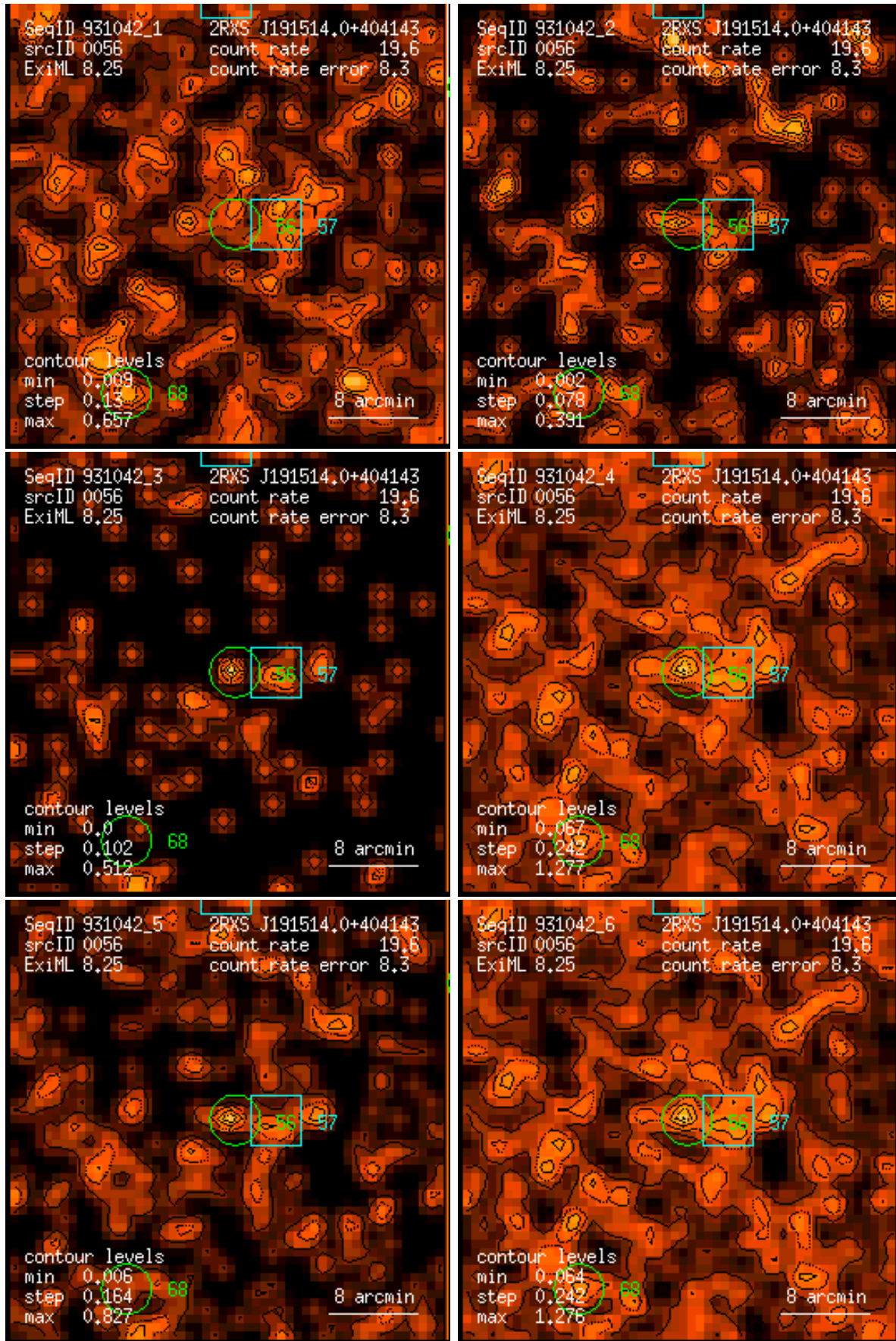
Figure 56: RASS 931042: detection 0056: band rate images, Gaussian filter: (1) PSPC channels 11 – 41, (2) 52 – 90, (3) 91 – 201, (4) 11 – 235, (5) 52 – 201, (6) 11 – 201. Broad band rates in counts/ks. Band rate contour levels in counts/ks/arcmin 2 .
