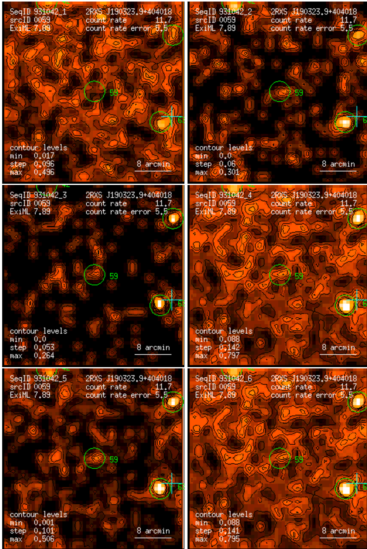
Figure 59: RASS 931042: detection 0059: band rate images, Gaussian filter: (1) PSPC channels 11 – 41, (2) 52 – 90, (3) 91 – 201, (4) 11 – 235, (5) 52 – 201, (6) 11 – 201. Broad band rates in counts/ks. Band rate contour levels in counts/ks/arcmin 2 .
