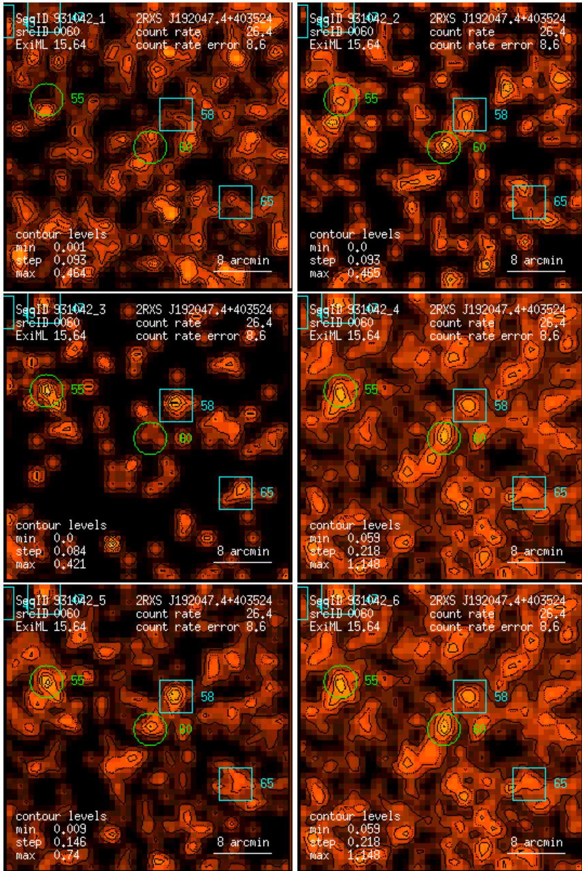
Figure 60: RASS 931042: detection 0060: band rate images, Gaussian filter: (1) PSPC channels 11 – 41, (2) 52 – 90, (3) 91 – 201, (4) 11 – 235, (5) 52 – 201, (6) 11 – 201. Broad band rates in counts/ks. Band rate contour levels in counts/ks/arcmin 2 .
