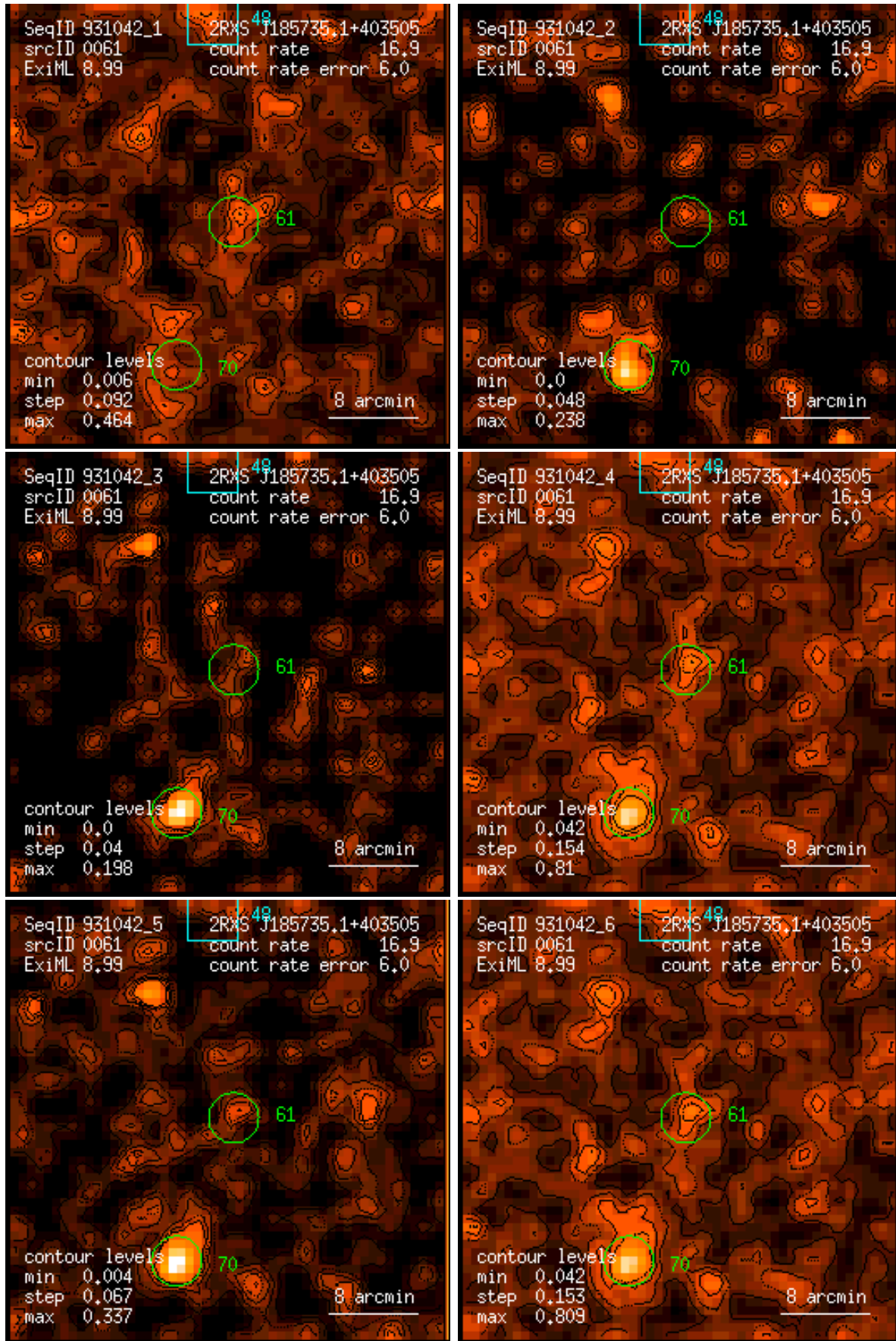
Figure 61: RASS 931042: detection 0061: band rate images, Gaussian filter: (1) PSPC channels 11 – 41, (2) 52 – 90, (3) 91 – 201, (4) 11 – 235, (5) 52 – 201, (6) 11 – 201. Broad band rates in counts/ks. Band rate contour levels in counts/ks/arcmin 2 .
