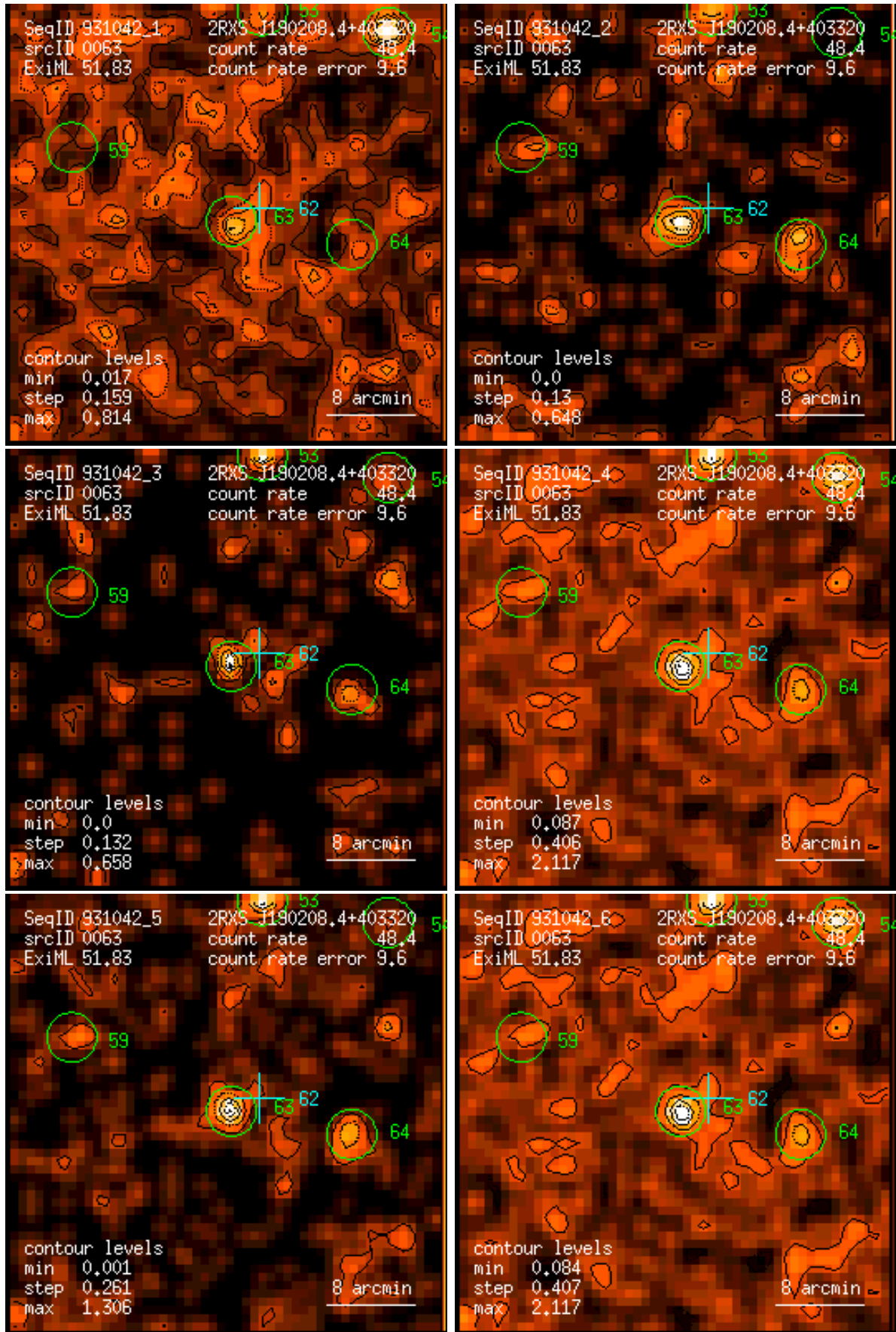
Figure 63: RASS 931042: detection 0063: band rate images, Gaussian filter: (1) PSPC channels 11 – 41, (2) 52 – 90, (3) 91 – 201, (4) 11 – 235, (5) 52 – 201, (6) 11 – 201. Broad band rates in counts/ks. Band rate contour levels in counts/ks/arcmin 2 .
