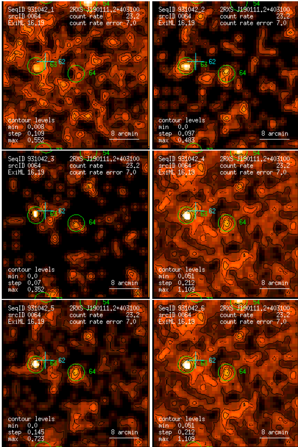
Figure 64: RASS 931042: detection 0064: band rate images, Gaussian filter: (1) PSPC channels 11 – 41, (2) 52 – 90, (3) 91 – 201, (4) 11 – 235, (5) 52 – 201, (6) 11 – 201. Broad band rates in counts/ks. Band rate contour levels in counts/ks/arcmin 2 .
